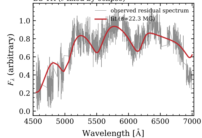
BS Tri ( \theta fixed by eclipse)
