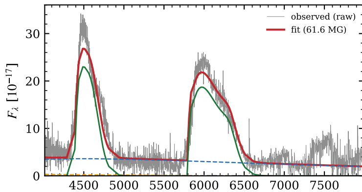
MQ Dra
