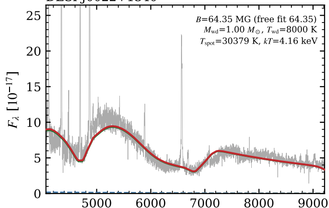
DESI J0022+1340
