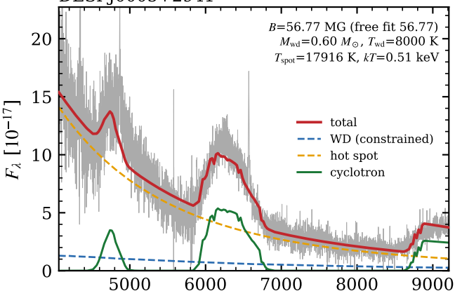
DESI J0005+2941
