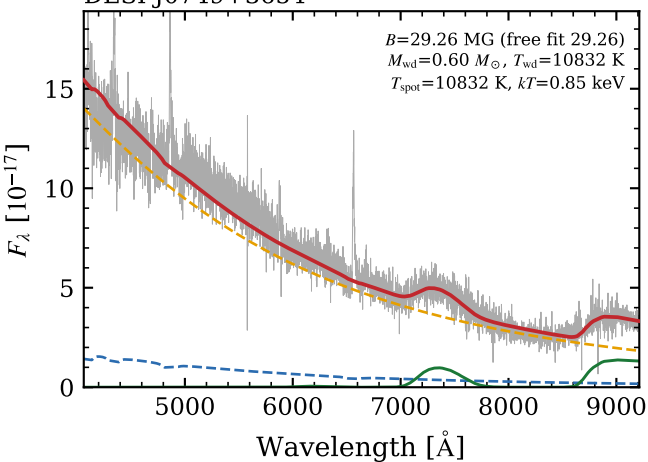
DESI J0749+3654
