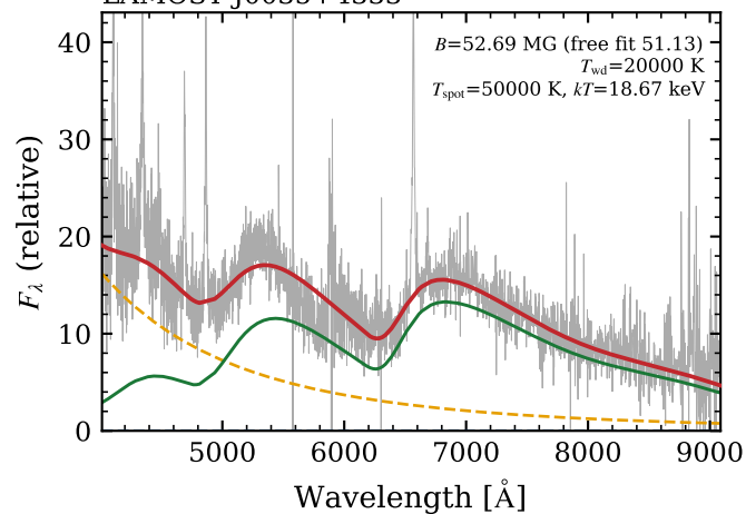
LAMOST J0035+4333
