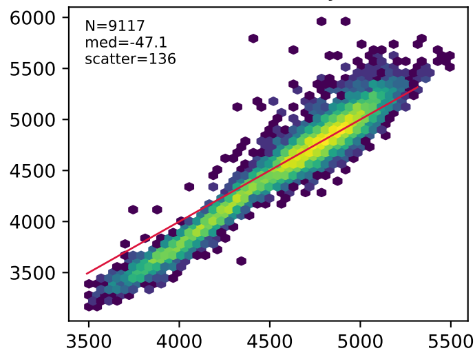
TransformerPayne
