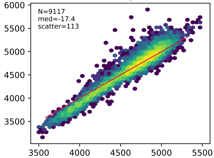
KAN-Payne
