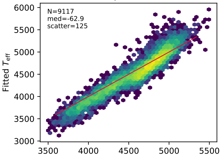
Payne-MLP
