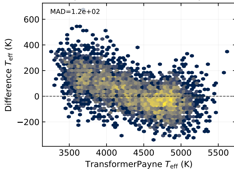
Payne-MLP - TransformerPayne
