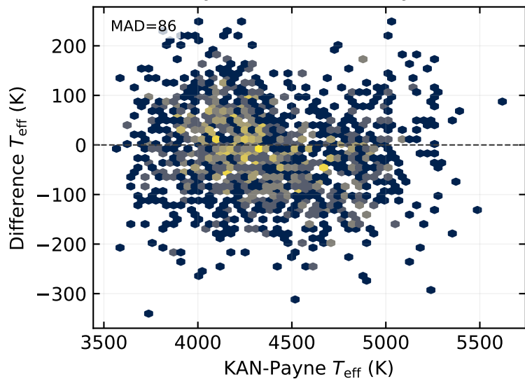
Payne-MLP - KAN-Payne
