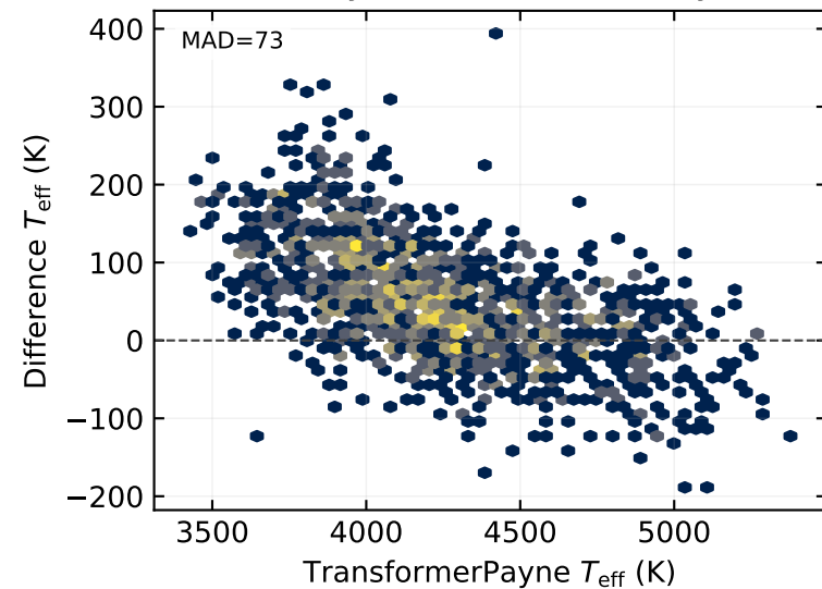
KAN-Payne - TransformerPayne
