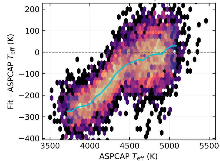
TransformerPayne
