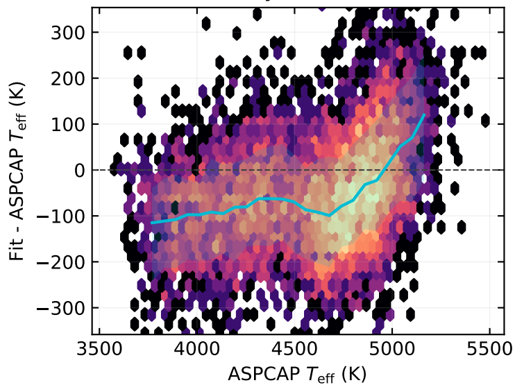
Payne-MLP
