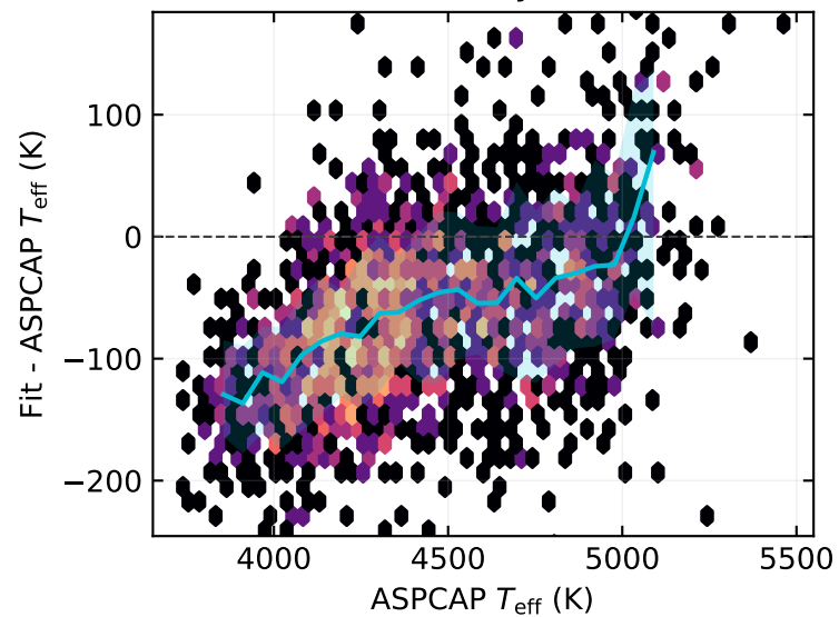
KAN-Payne
