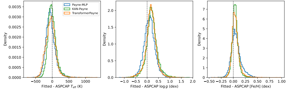
Figure 6. APOGEE DR17 residual distributions for the atmospheric labels. The narrower KAN-Payne [\text{Fe}/\text{H}] distribution is consistent with the synthetic-grid validation result and indicates that the KAN emulator improves the forward model in abundance-sensitive spectral regions on the common quality sample.
