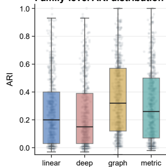
d Family-level ARI distribution
