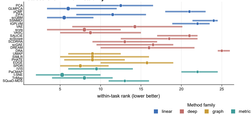
g Dataset-level ARI rank stability
