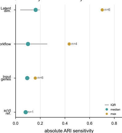
i Control-layer ARI sensitivity
