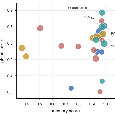
e Global score versus memory
