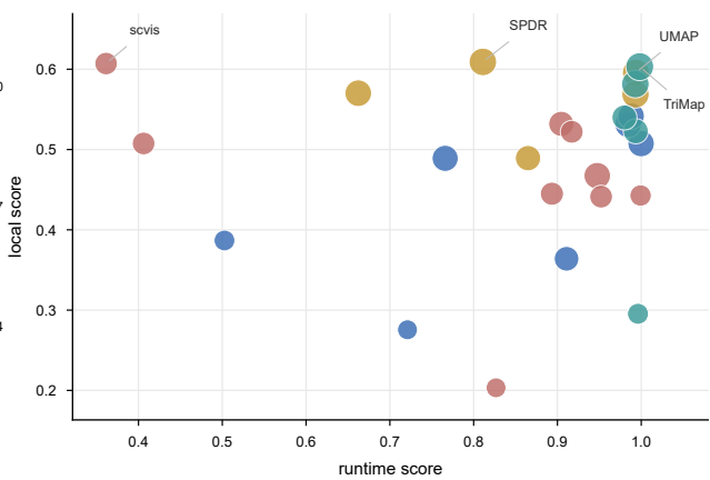
d Local score versus runtime
