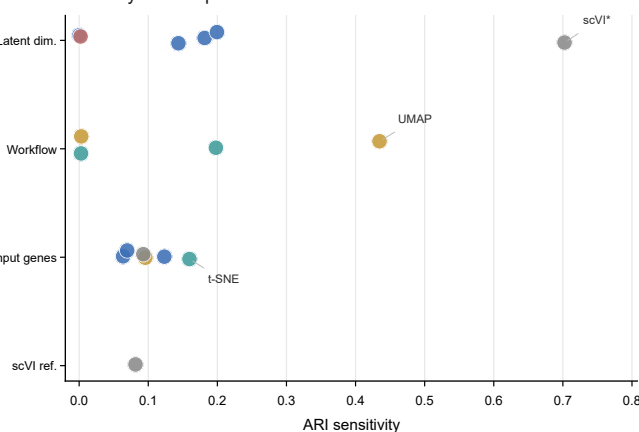
j Sensitivity landscape
