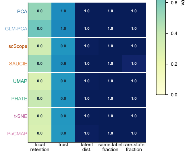
f Rare population
