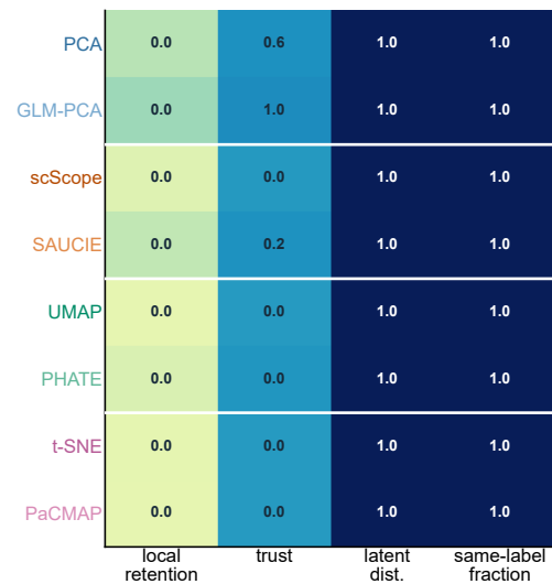
d Dropout stress
