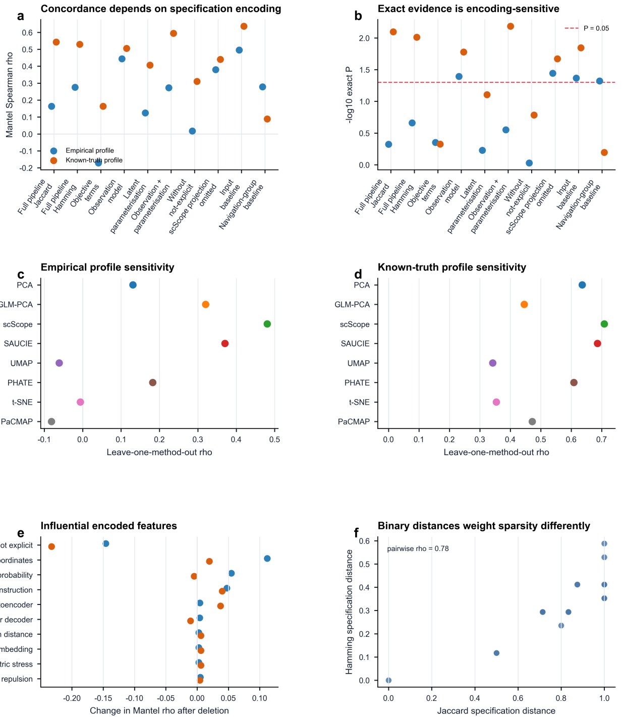
Supplementary Fig. S9. Specification-to-profile concordance depends on encoding and method composition. a , Exact Mantel Spearman correlation between ten alternative specification encodings and the empirical or controlled-scenario profile. Each point uses eight methods and 28 unique method pairs. b , Negative base-10 logarithm of the corresponding exact two-sided P value; the dashed line marks unadjusted P = 0.05 . Alternative encodings are exploratory and were not selected by these P values. c , d , Leave-one-method-out Mantel correlations for empirical and controlled-scenario profiles. Each point uses seven methods, 21 pairs and all 5,040 method-label permutations. e , Change in Mantel correlation after deleting one encoded feature from the full specification; the ten features with the largest absolute change across the two profiles are shown. f , Jaccard against Hamming distance for the 28 method pairs under the same 17-feature encoding. The displayed Spearman correlation describes the pairwise relation and is not an independent-pair significance test. Blue and orange identify empirical and controlled-scenario profiles. Complete encodings and exact permutation results are reported in Supplementary Table S9.
