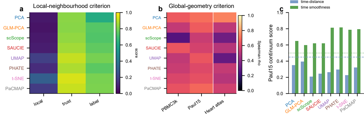
Continuum criterion
