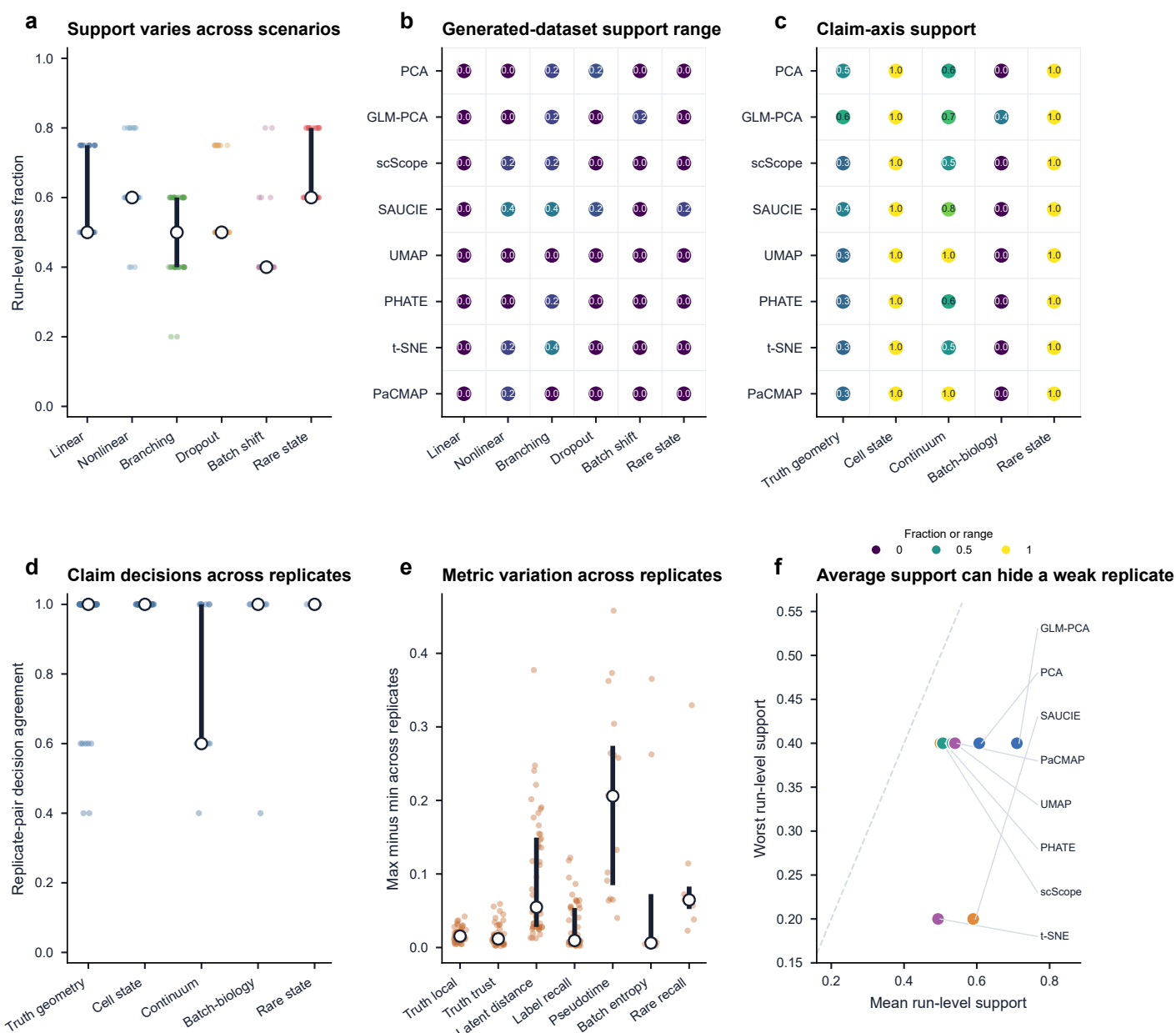
Supplementary Fig. S13. Five independently generated datasets per scenario quantify controlled stress-test stability. a, Run-level support fraction across 40 runs for each scenario, comprising eight methods and five generated datasets. Small points are runs; open circles are medians and vertical bars span interquartile ranges. b, Range in run-level support across the five generated datasets for every method-scenario combination. In-cell values give the range from 0 to 1. c, Interpretation-axis pass fraction for every method across all applicable generated-dataset metric rows. Point colour and label encode the fraction. d, Metric-specific decision agreement for the ten shared pairs formed from five generated datasets for generating-structure geometry, cell state, continuum, batch-biology trade-off and rare-state interpretations. e, Maximum-minus-minimum metric value across generated datasets for each method-scenario-metric combination; points are combinations and open circles are medians and bars span interquartile ranges. f, Mean run-level support against worst-run support for each method. The dashed diagonal marks equality, and connectors associate displaced labels with points. Generated datasets are computational replications rather than biological replicates; shared pairs are not independent repetitions. The analysis contains 30 generated datasets, 240 complete runs and 1,120 valid metric rows; complete results are reported in Supplementary Table S13.
