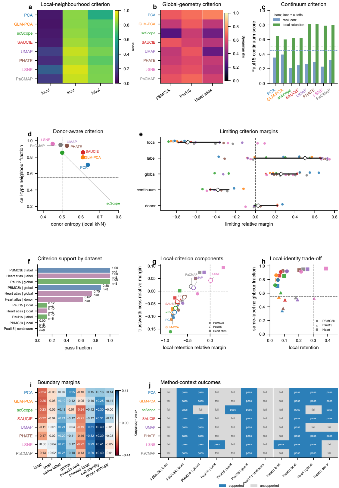
Supplementary Fig. S14. Operational diagnostic criteria and threshold sensitivity in the eight-method anchor panel. a , Mean local retention, trustworthiness and same-label neighbour fraction across PBMC3k, Paul15 and the heart subset for each method. b , Global-rank correlation by method and dataset. c , Paul15 pseudotime-distance correlation and local pseudotime retention under the stored 8Mk-root definition; dashed lines mark operational boundaries of 0.45 and 0.50. d , Heart-subset donor entropy and same-label-type-neighbour fraction; dashed lines mark operational boundaries of 0.50 and 0.55, and the grey connector associates the displaced scScope label with its point. e , Limiting signed relative margin for each applicable method-context-claim decision, defined as the smallest component value of (\text{value} - \text{boundary}) / \text{boundary} within a criterion. Coloured points are decisions, black segments span the interquartile range, open diamonds are medians and the dashed line marks zero. f , Criterion support by dataset and claim; labels report the supported fraction and number of evaluated method rows. g , Joint local-criterion component plane for 24 method-context evaluations. Solid points are individual evaluations, open circles are method means, colour identifies method and symbol identifies dataset. h , Local retention against same-label neighbour fraction for the same 24 runs. i , Mean observed-minus-boundary margin for each method and diagnostic component. j , Binary outcomes for all applicable method-context-claim criteria; blank combinations were not defined and were not counted as failures. The boundaries are study-level operational decision rules, not statistical significance thresholds or universal performance standards. Continuous values and margins are the primary evidence; the binary summaries are retained for sensitivity and auditability.
