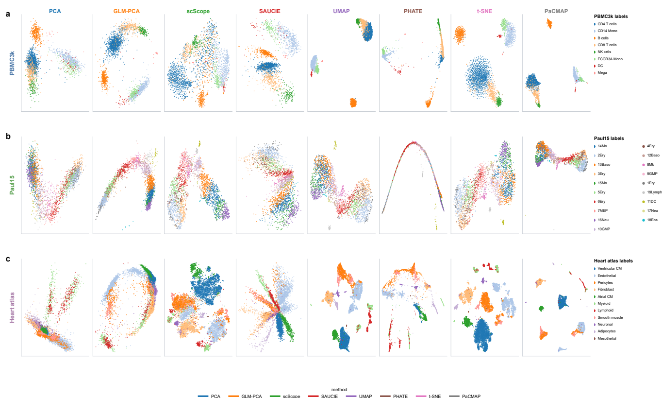
Supplementary Fig. S3. Full embedding atlas across empirical interpretation contexts. a-c, Low-dimensional coordinates for the eight-anchor empirical panel in PBMC3k, Paul15 and the heart-atlas subset. Columns show PCA, GLM-PCA, scScope, SAUCIE, UMAP, PHATE, t-SNE and PaCMAP in the same fixed order used throughout the study. Points are cells and colours denote the dataset-specific annotation labels shown at the right of each row. Method-name colours are navigational identifiers only and do not encode a method class or performance level. These maps document the fitted coordinates underlying the matched comparisons; visual separation is not used as a quantitative result. Diagnostics and biological-consistency checks are reported in Figs 3-5. Here, n is the number of cells in the processed analysis object for each dataset-method map; fitted coordinates and plotting code are available in the public repository.
