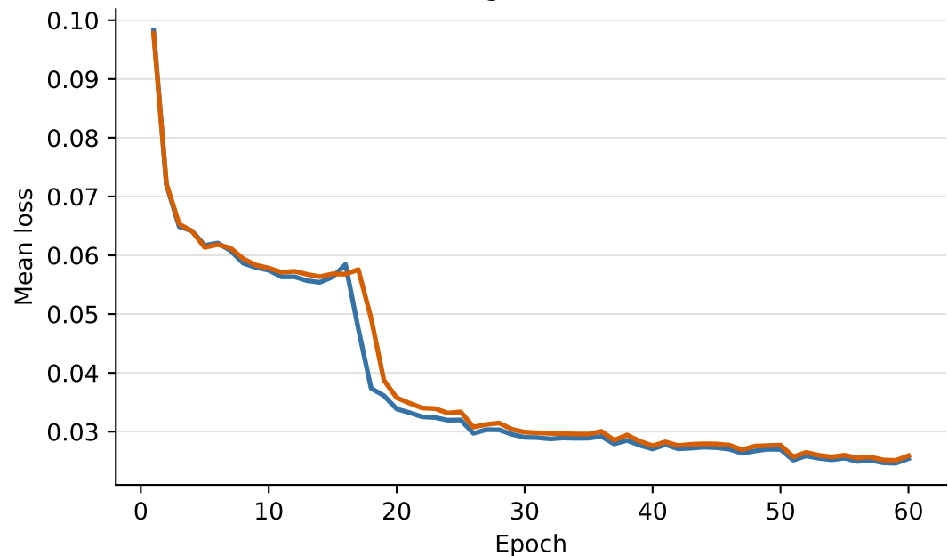
Sobel-gradient loss
