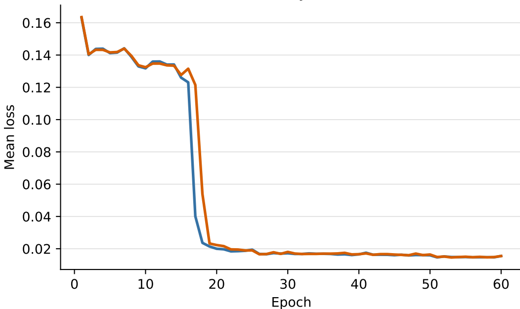
Intensity loss
