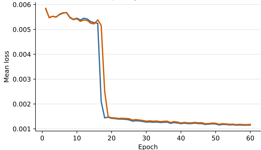
Sobel-gradient loss
