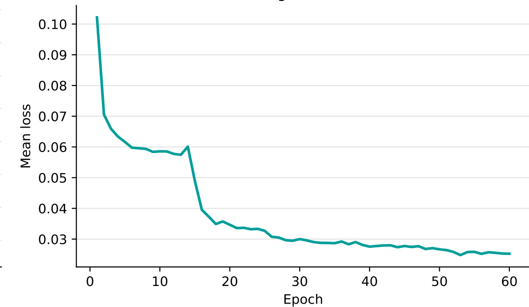
Sobel-gradient loss
