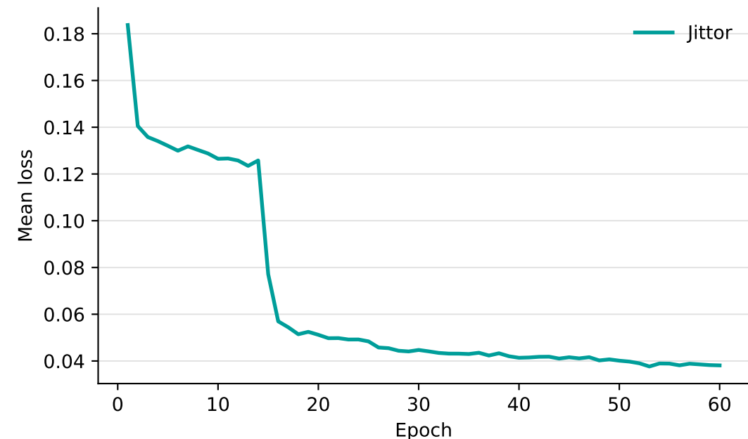
Intensity loss
