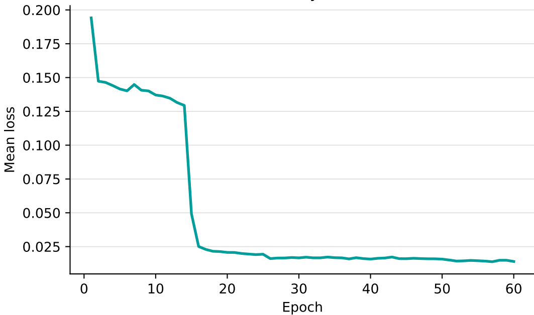
Intensity loss
