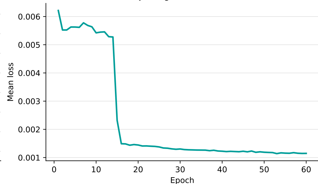
Sobel-gradient loss
