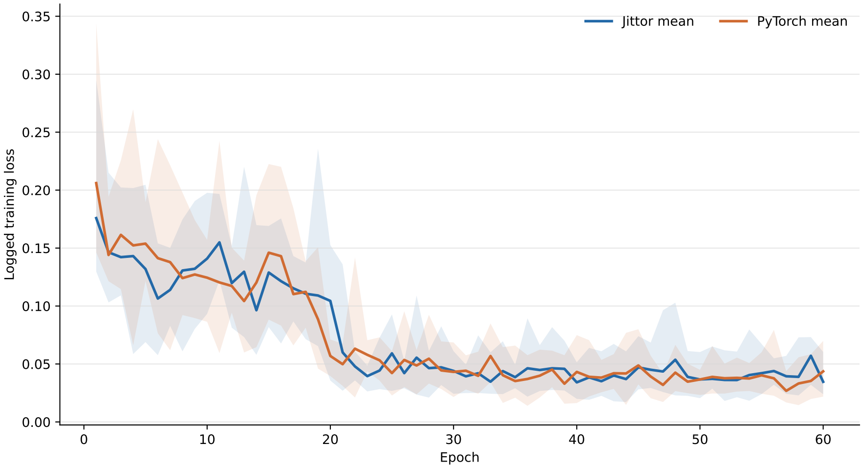
SIBA training loss (official logging interval: every 50 batches)
