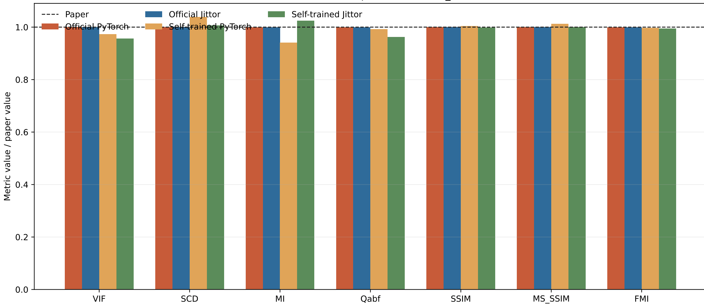
SIBA metric comparison on M3FD_2x
