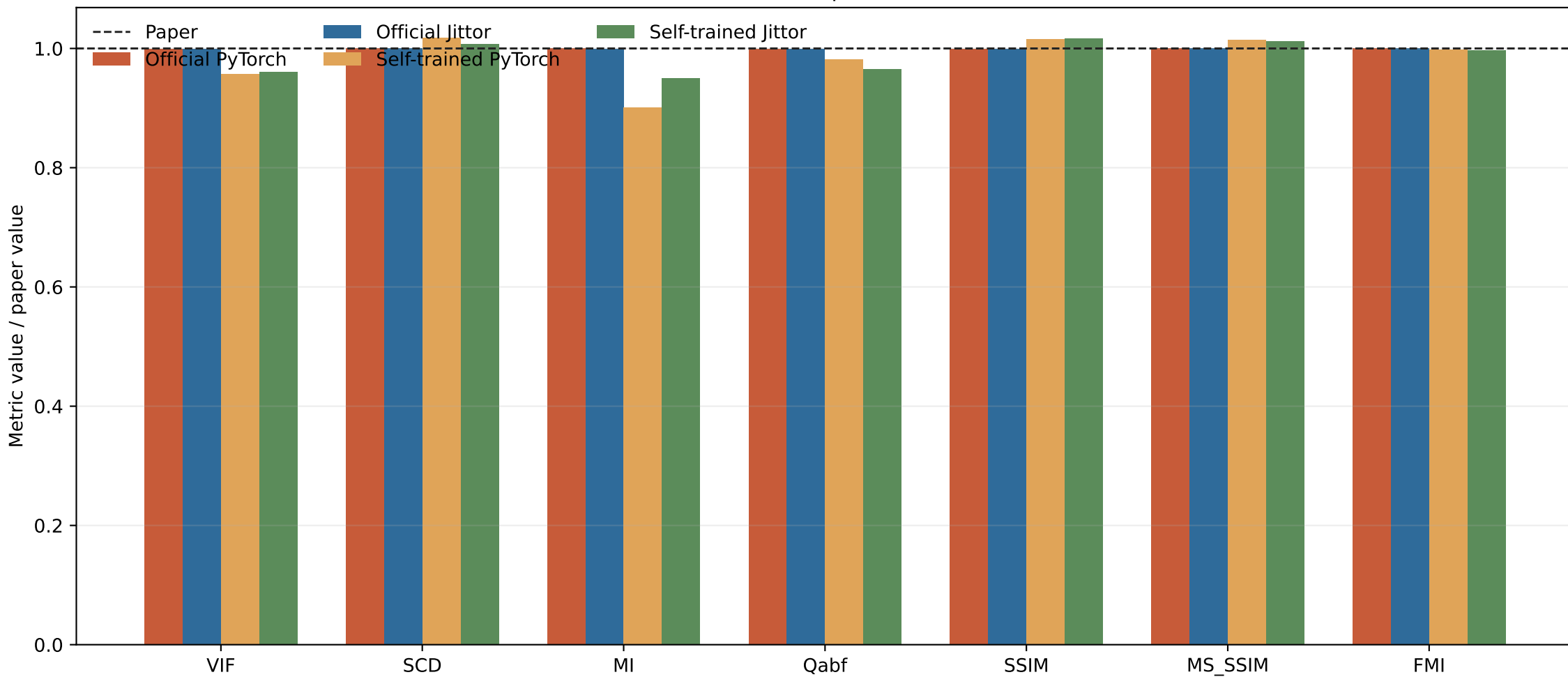
SIBA metric comparison on TNO
