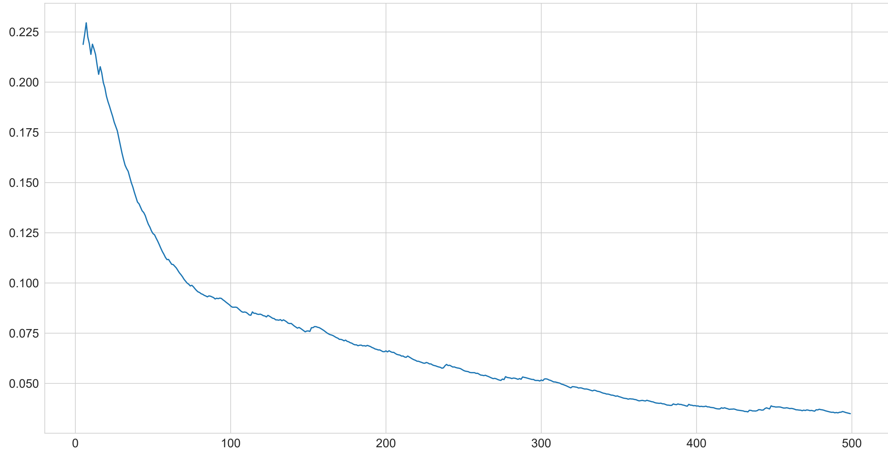
DAE loss
