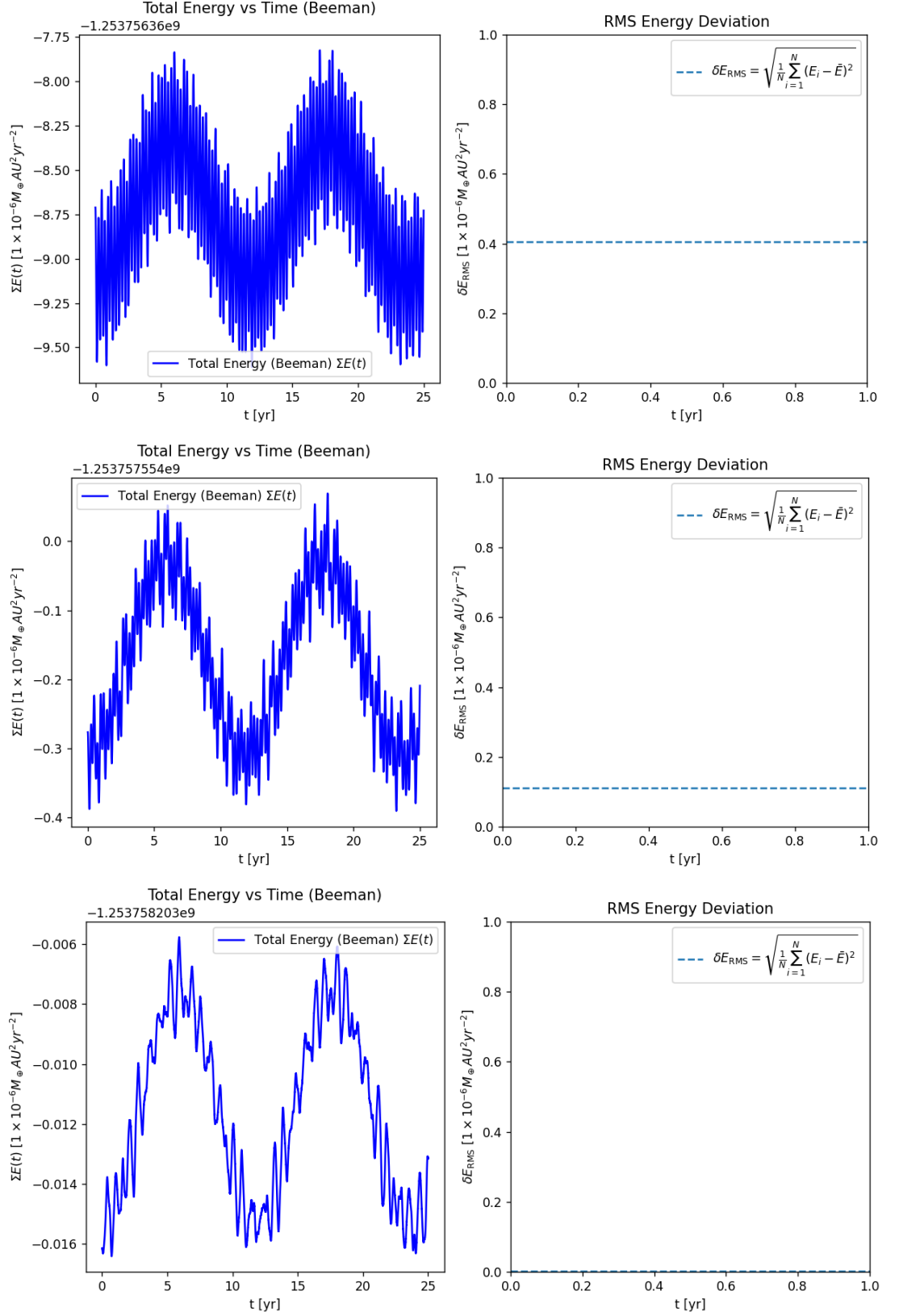
Figure 5. Total energy \Sigma E(t) vs time and \delta E_{RMS} graphs for Beeman integration at dt = 0.001 (top graph), 0.0006 (middle graph) and 0.0001 (bottom graph) in [yr]. Evidence of \delta E_{RMS} decreasing as dt shrinks.
