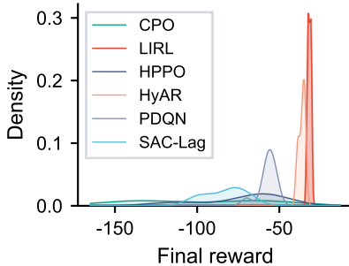
Reward distribution
