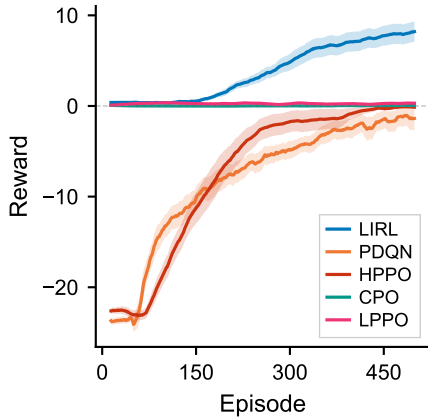
Learning curve
