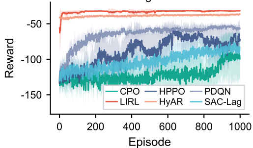
Training curves
