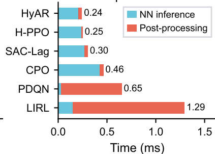
Computation time
