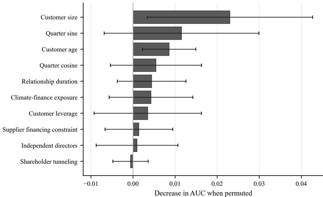
Permutation importance in the 2022-2023 holdout
