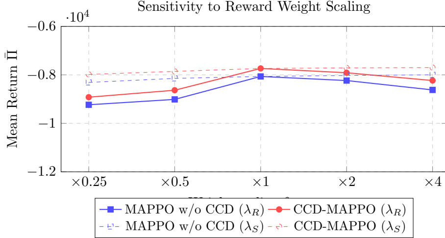
Figure 6: Sensitivity of mean return \bar{\Pi} to reward weight scaling. Solid lines: varying \lambda_R ; dashed lines: varying \lambda_S . ( \lambda_C curves are omitted for visual clarity; they show a similar pattern to \lambda_S with smaller magnitude.) The CCD-MAPPO advantage holds throughout the sweep.
