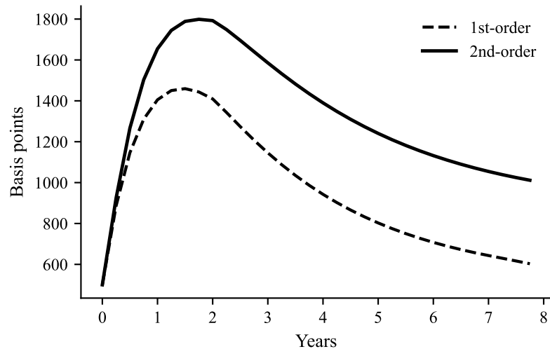
Panel D. Linearization bias (peak GDP)
