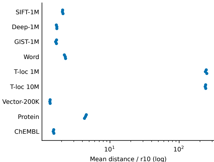
Representation sparsity
