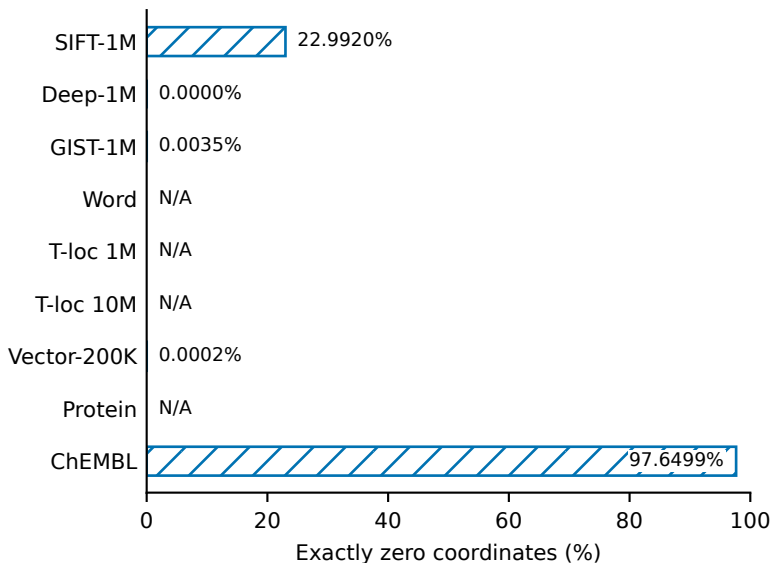
Representation sparsity
