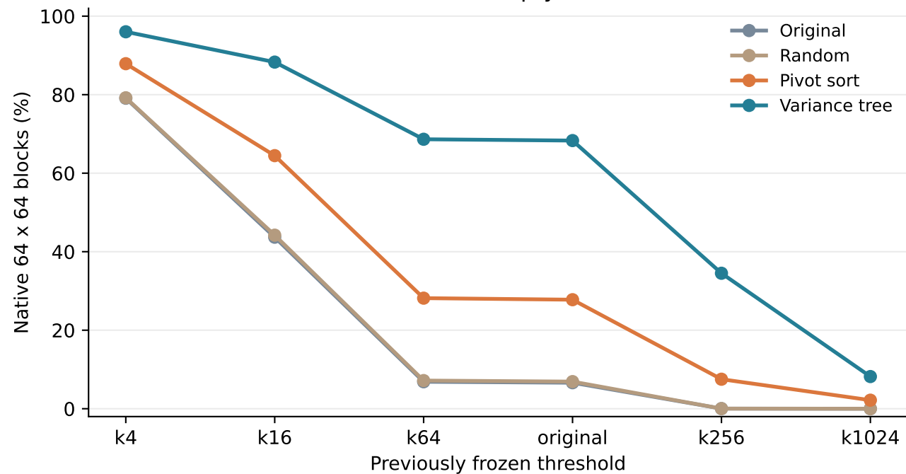
Answer-informed empty-block census
