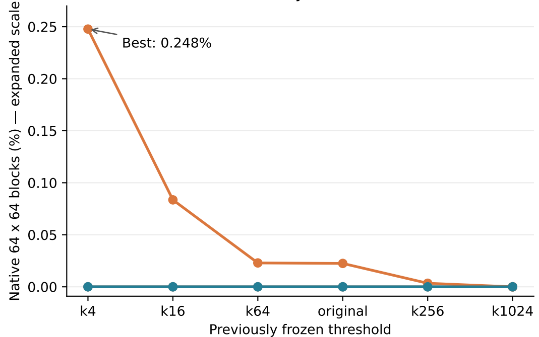
Blocks identified by combined bounds
