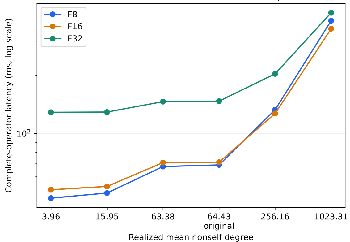
Fixed methods with the same GPU output
