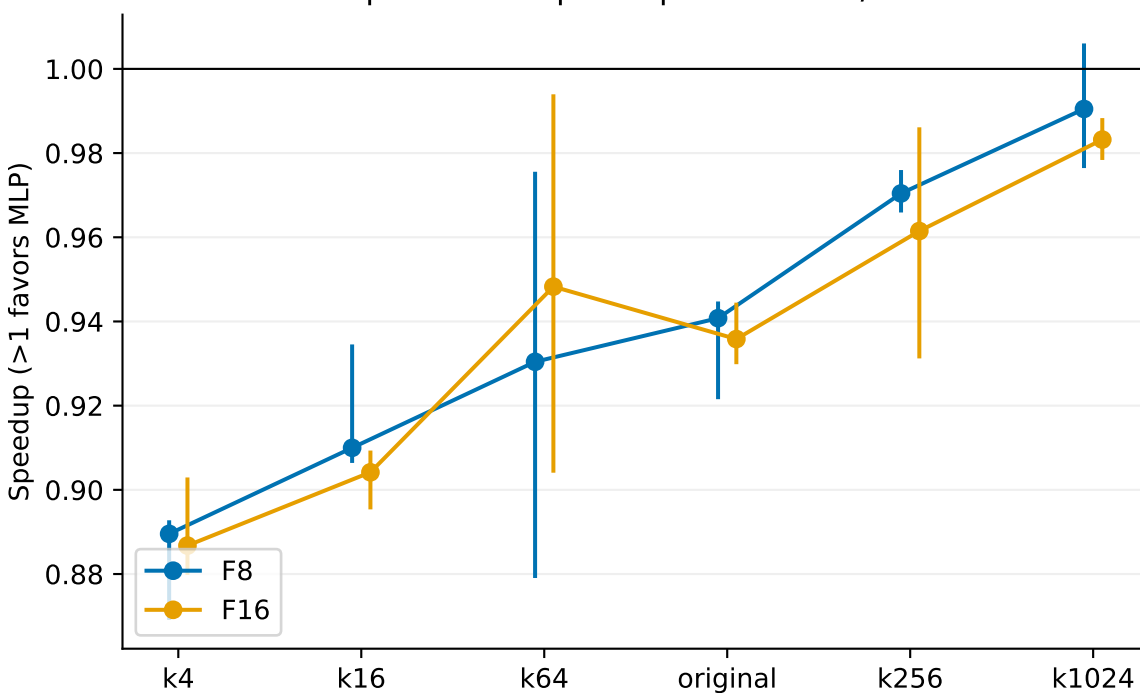
Repeated complete queries: PCA / MLP
