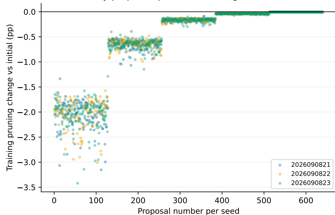
Equal-six-query mixture, this round only
