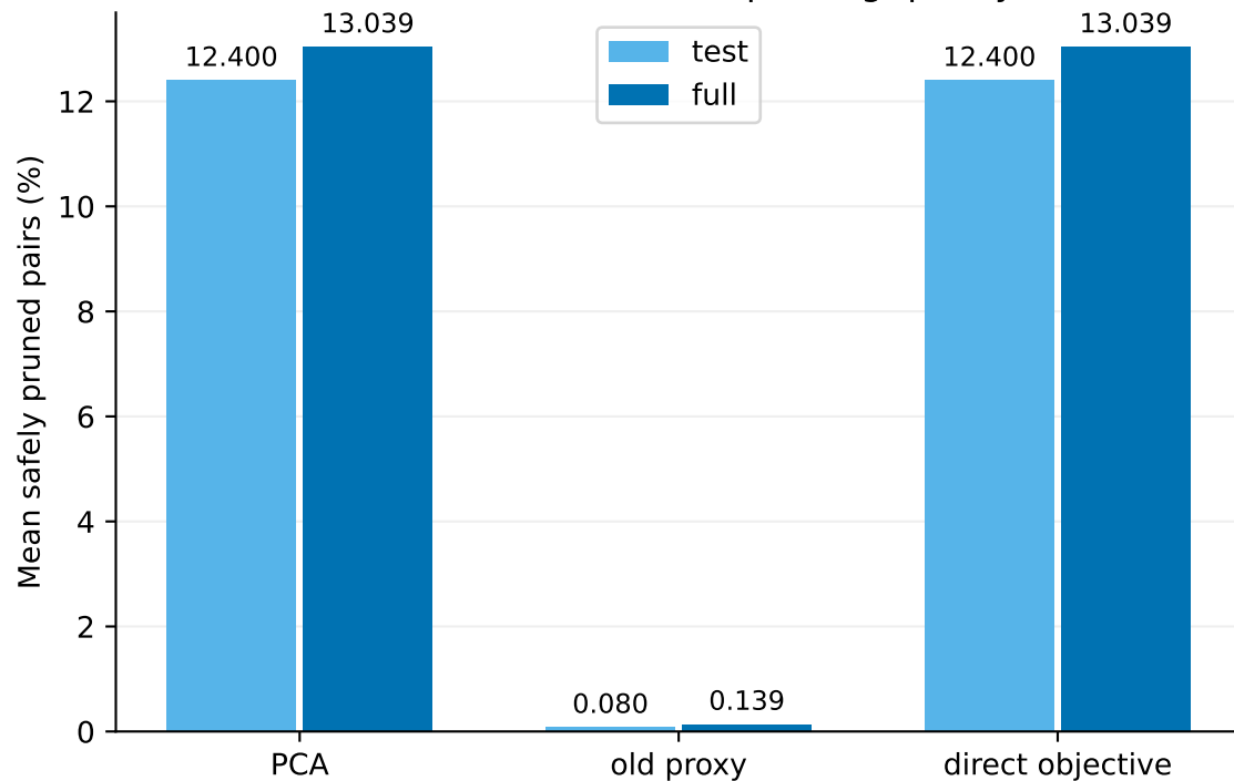
Same certified bound: pruning quality
