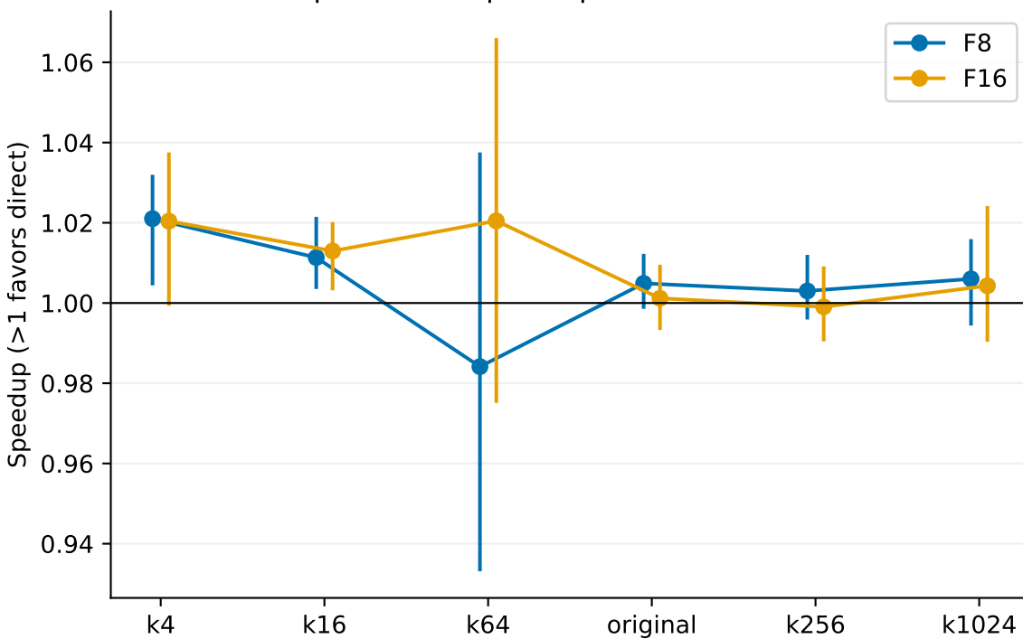
Repeated complete queries: PCA / direct
