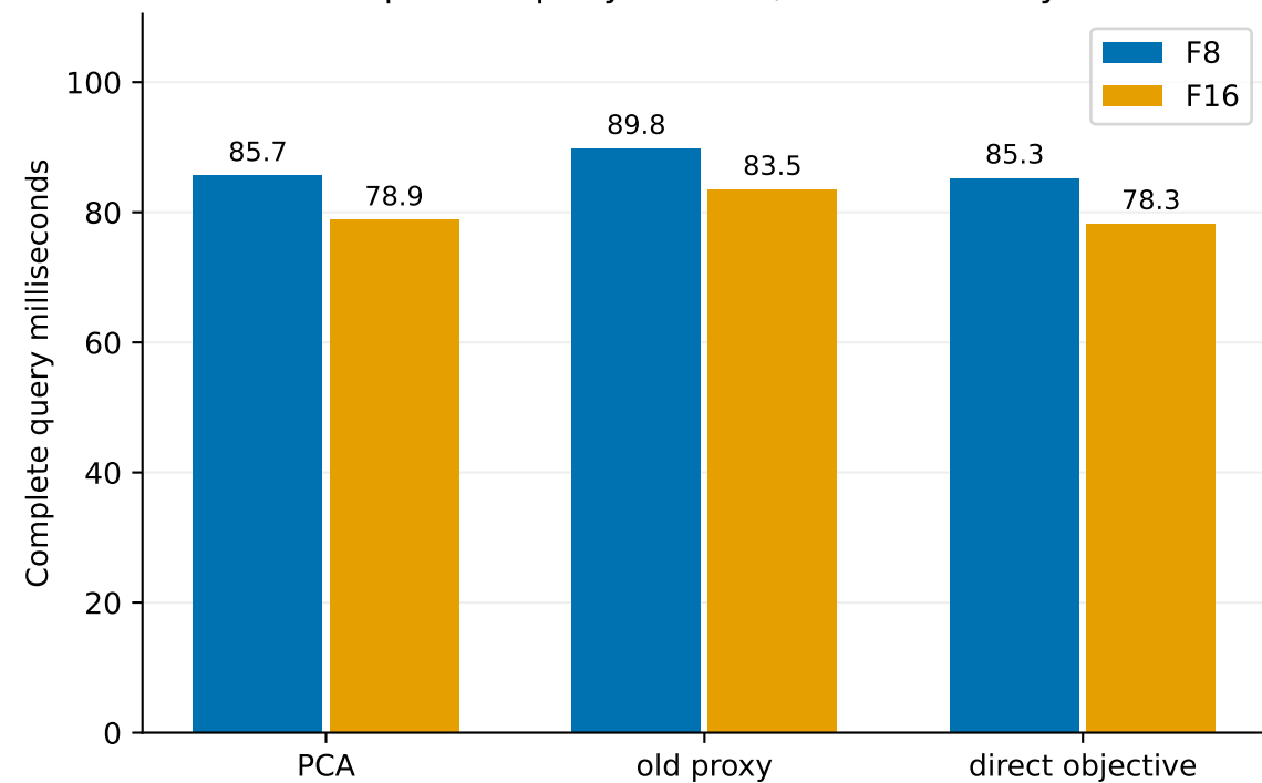
Equal-six-query mixture, this round only
