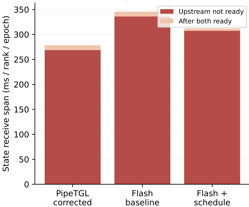
A State dependency, 8 GPUs
