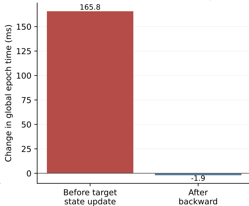
B Add 1 ms of CUDA latency
