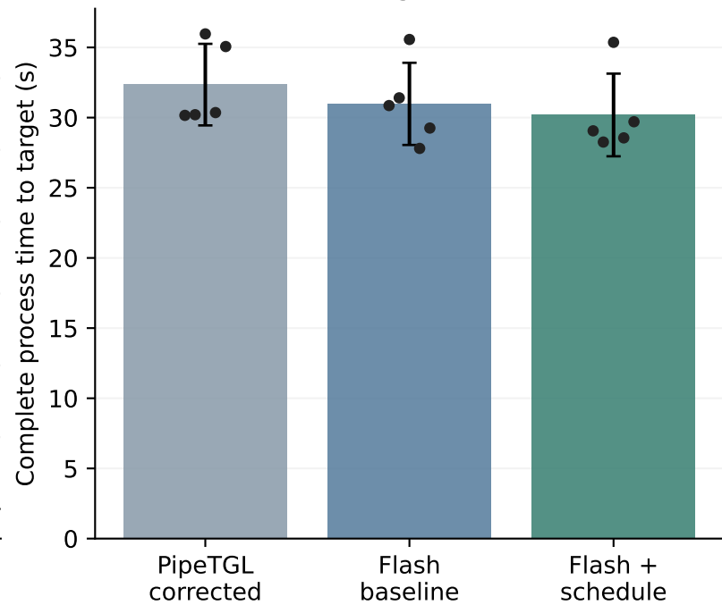
C Same AP target, 5 new seeds
