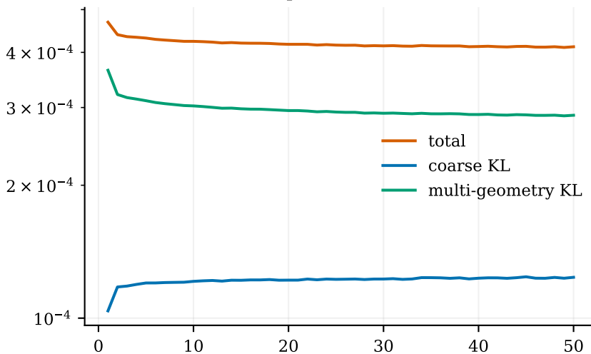
Spatial losses
