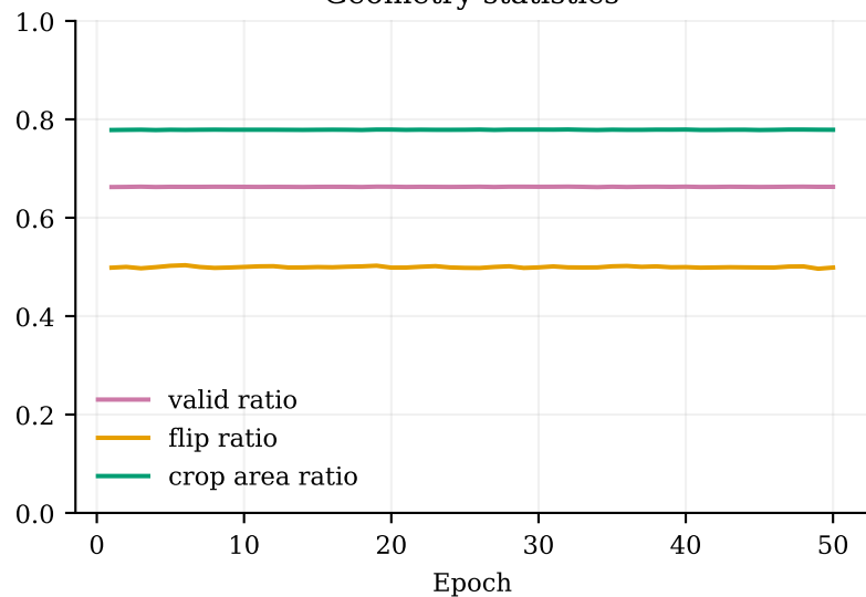
Geometry statistics
