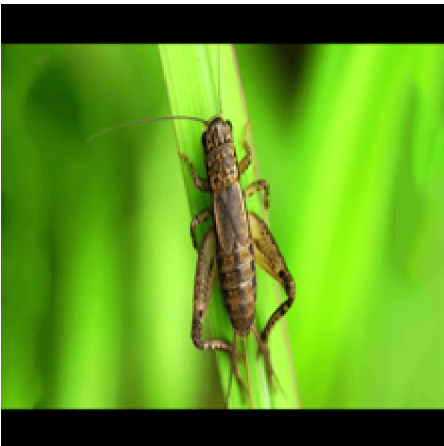
L3 affinity (14×14)
