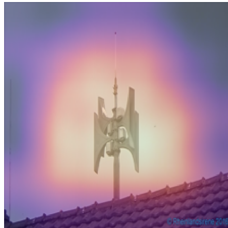
Pooled refined (7×7)
