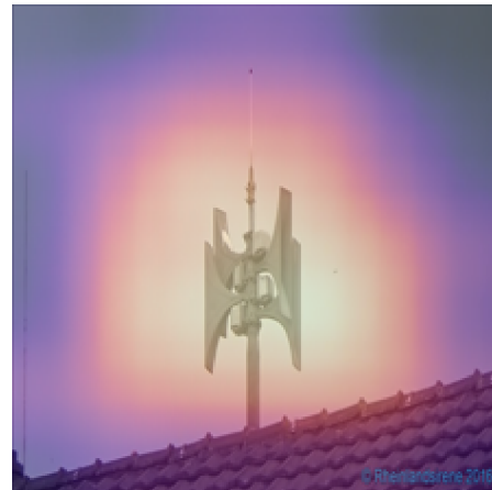
Native – pooled
