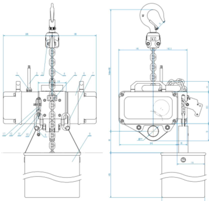
SINGLE-BRAKE CONFIGURATION
