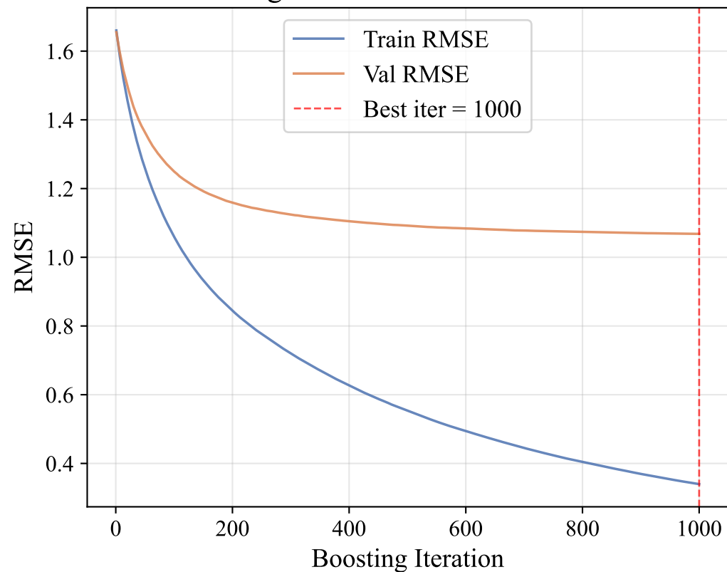
Training & Validation Loss — KCAT
