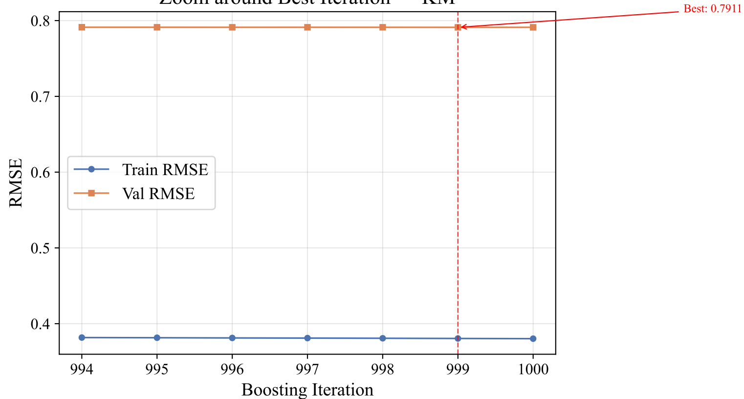
Zoom around Best Iteration — KM
