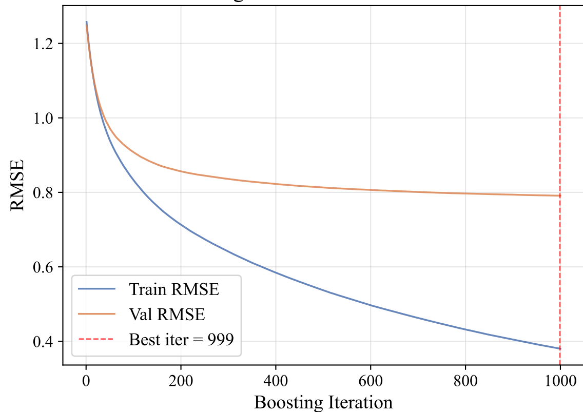
Training & Validation Loss — KM
