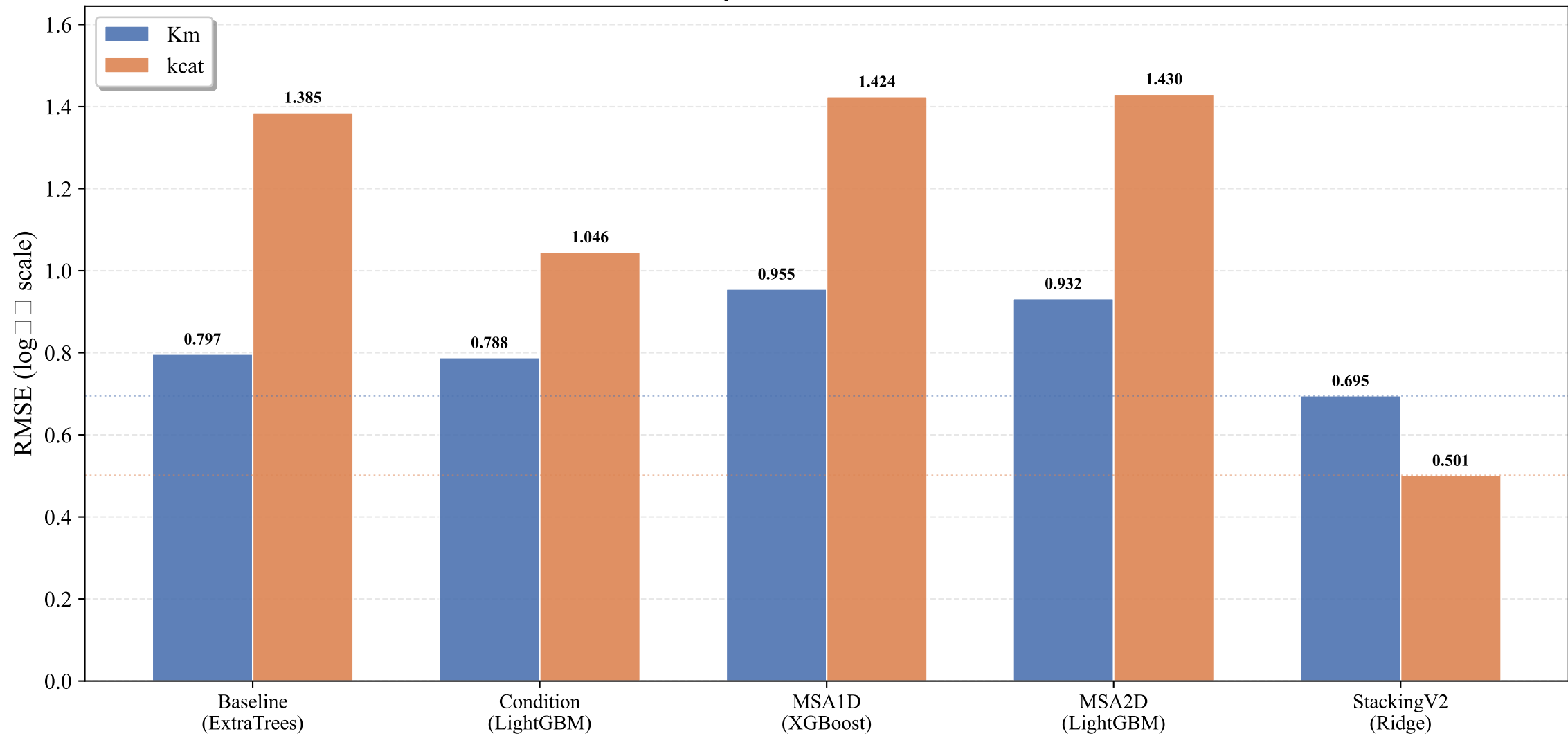
Model Comparison — RMSE on Test Set
