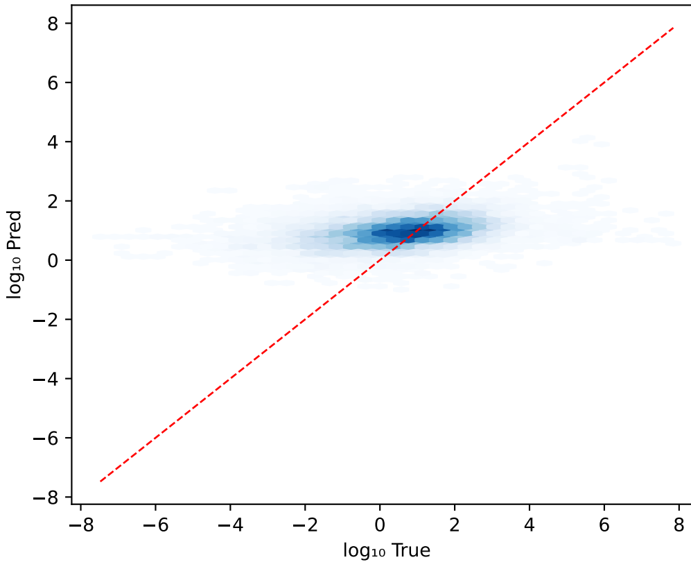
kcat: Pred vs Exp R 2 =-0.000
