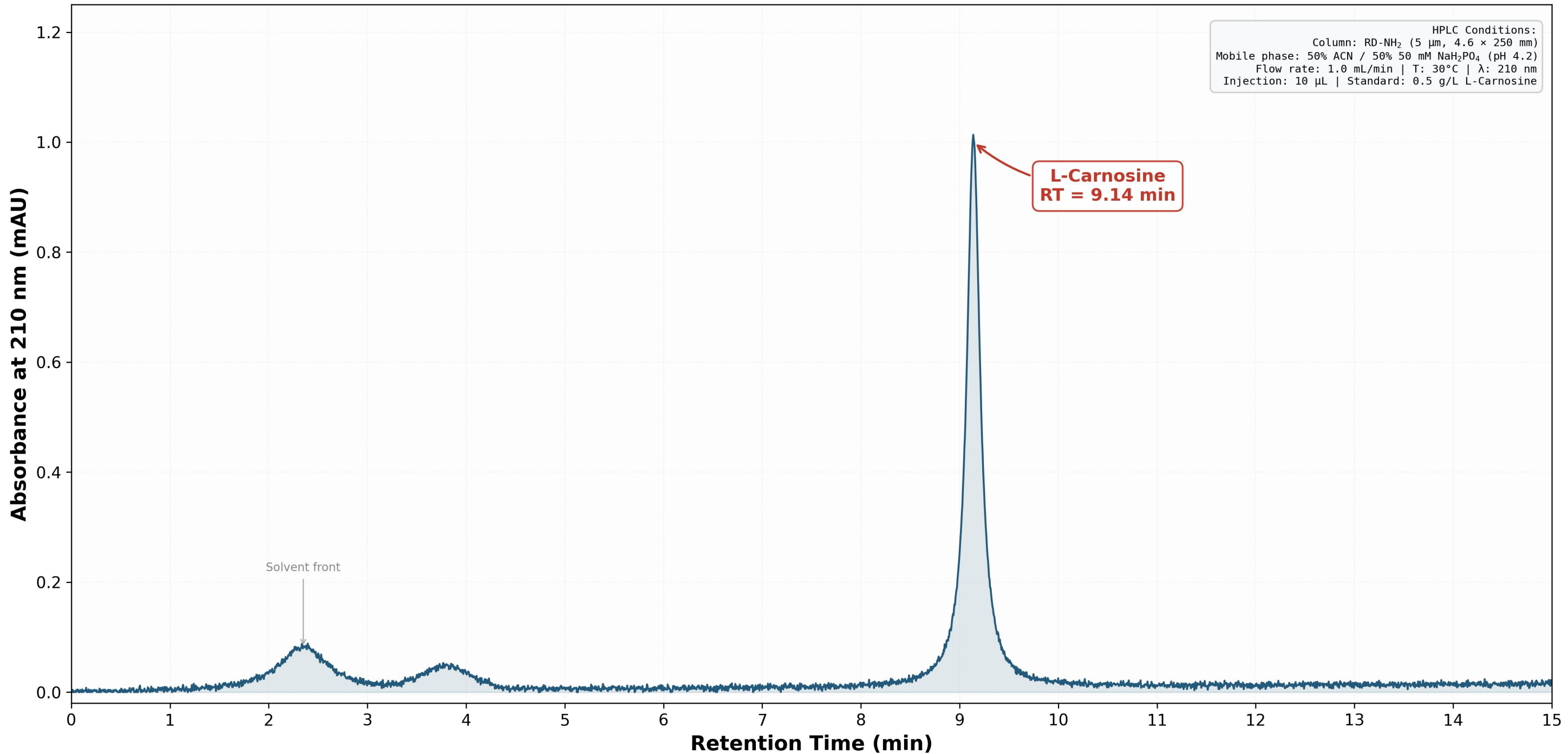
Figure 1. HPLC Chromatogram of L-Carnosine Standard
