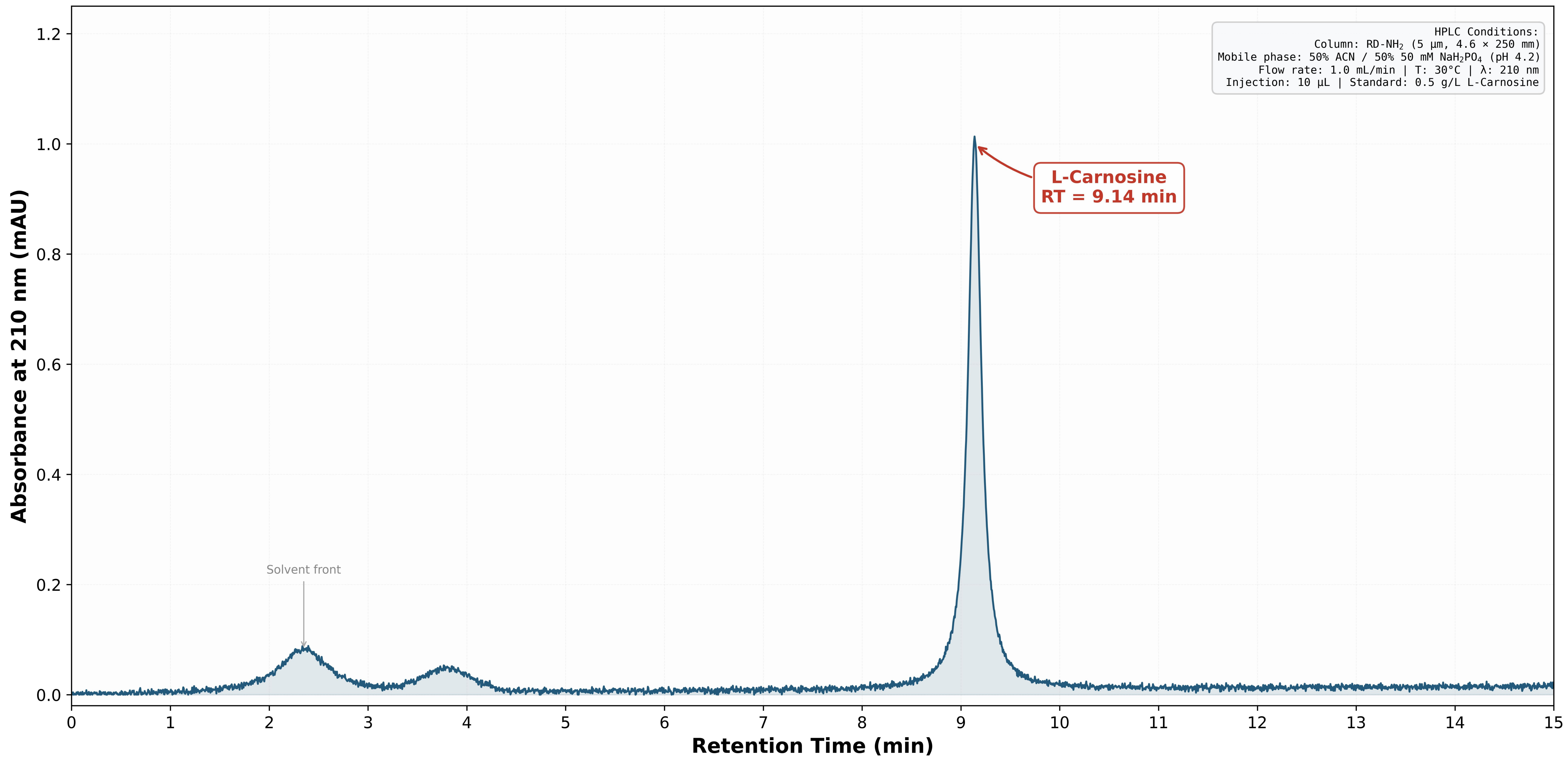
Figure 1. HPLC Chromatogram of L-Carnosine Standard
