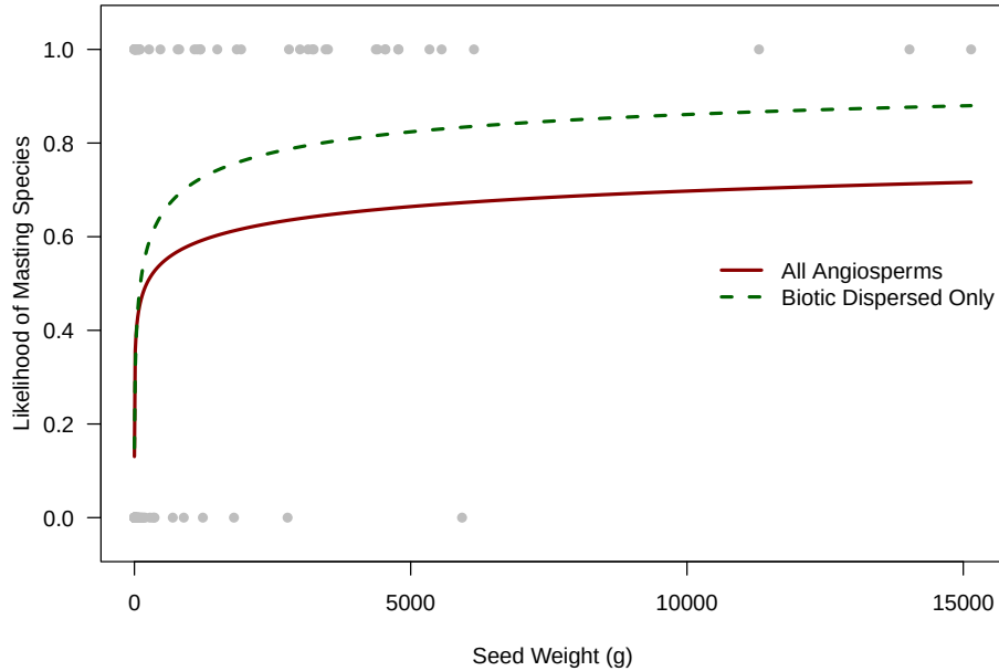
Figure 3: Predicted likelihood of masting as a function of seed mass for all angiosperm species (solid red line) and the biotic-dispersed subgroup (dashed green line), estimated using phylogenetic logistic regression (phyloglm). Individual species observations are plotted as binary data points at 0 (non-masting) and 1 (masting).
