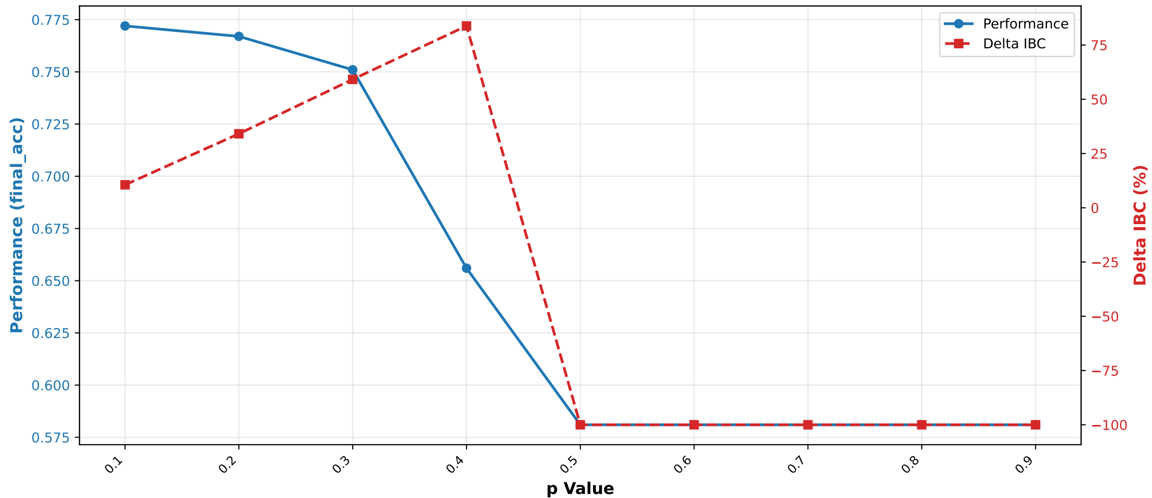
CNLI_SHORT - Neural Router Results Performance vs Delta IBC
