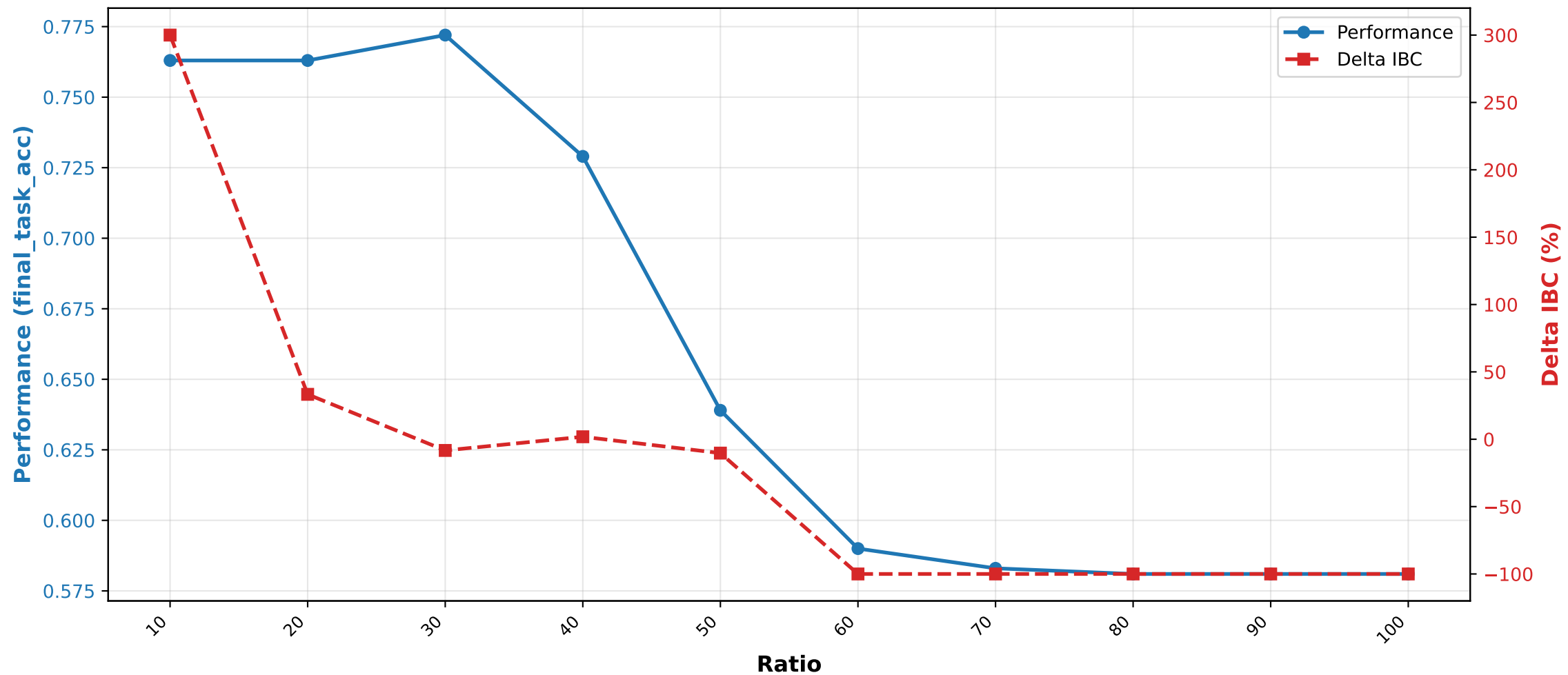
CNLI_SHORT - POMDP Logits Results Performance vs Delta IBC
