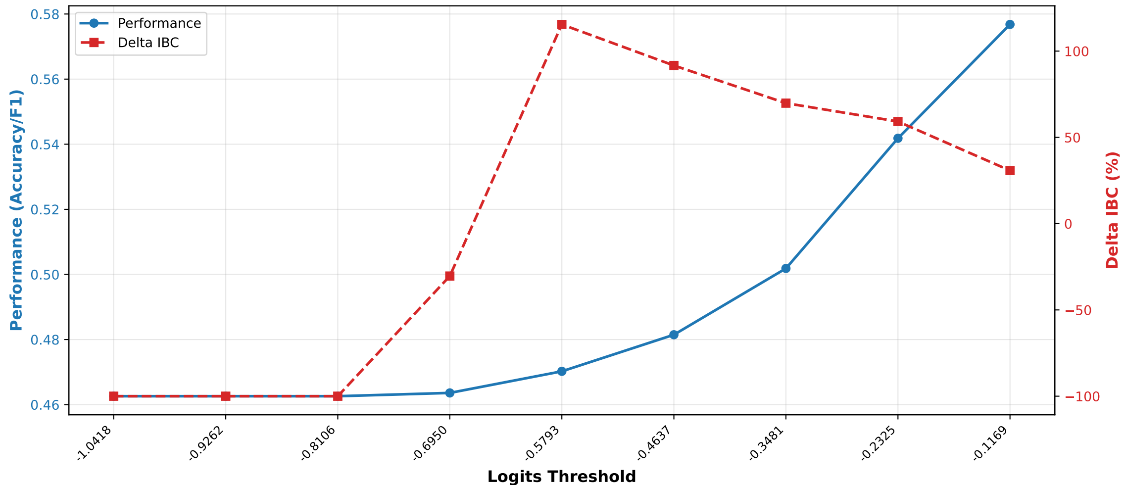
COQA_SHORT - Logits Thresholds Performance vs Delta IBC
