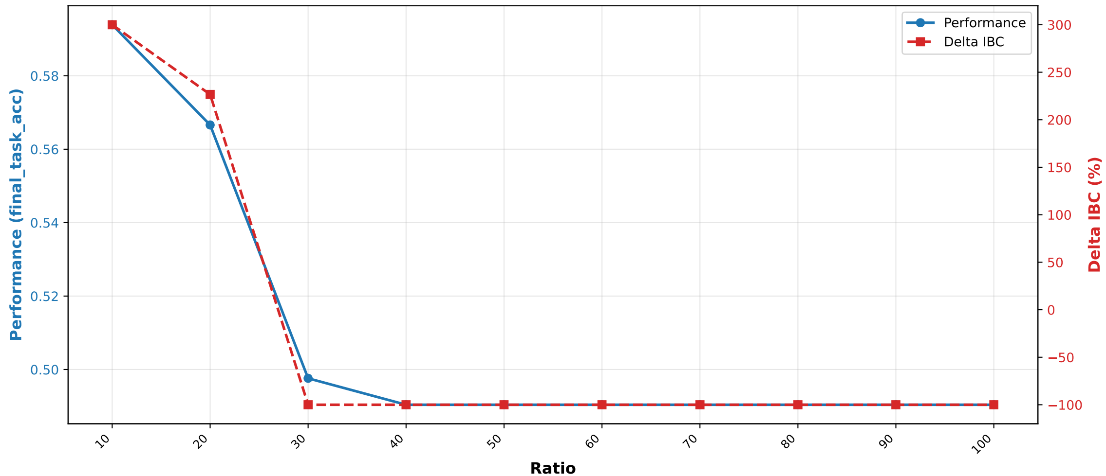
COQA_SHORT - POMDP Logits Results Performance vs Delta IBC
