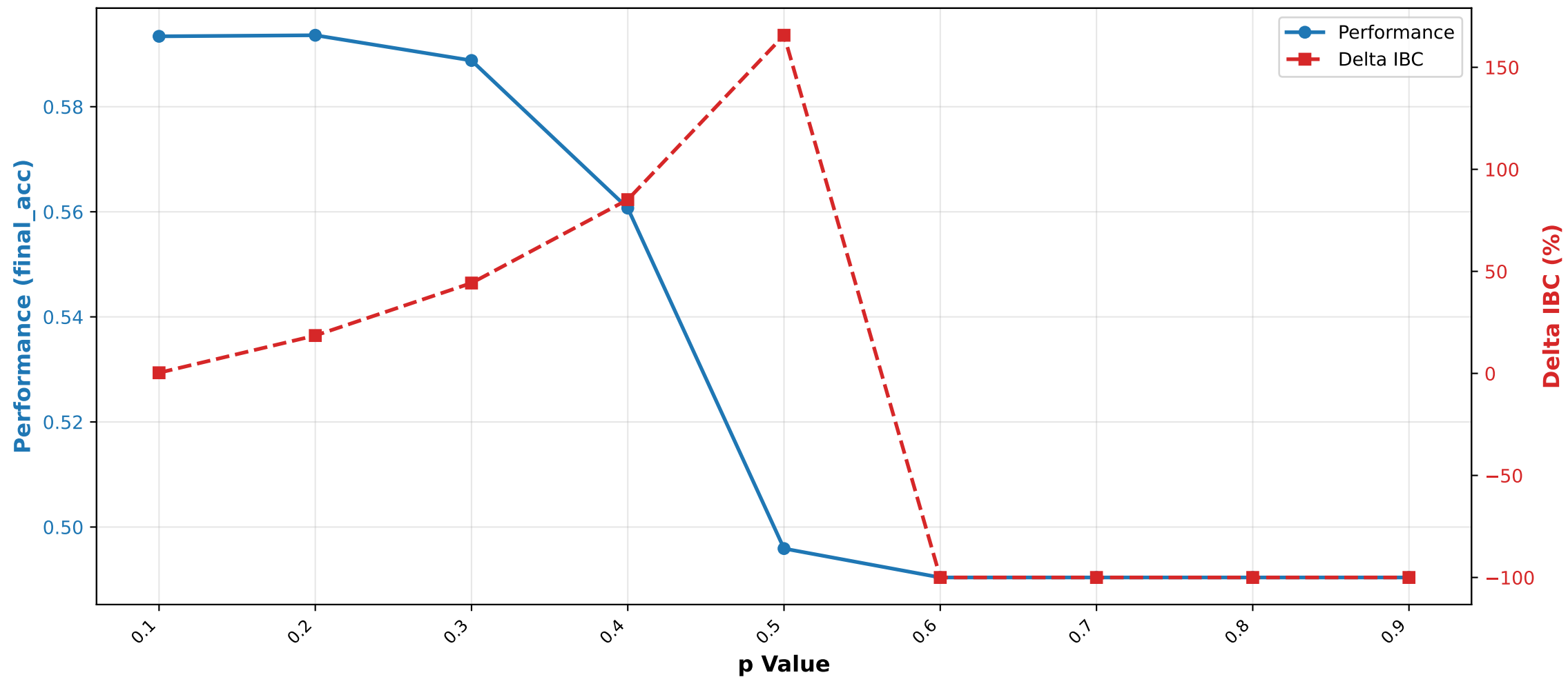
COQA_SHORT - Neural Router Results Performance vs Delta IBC
