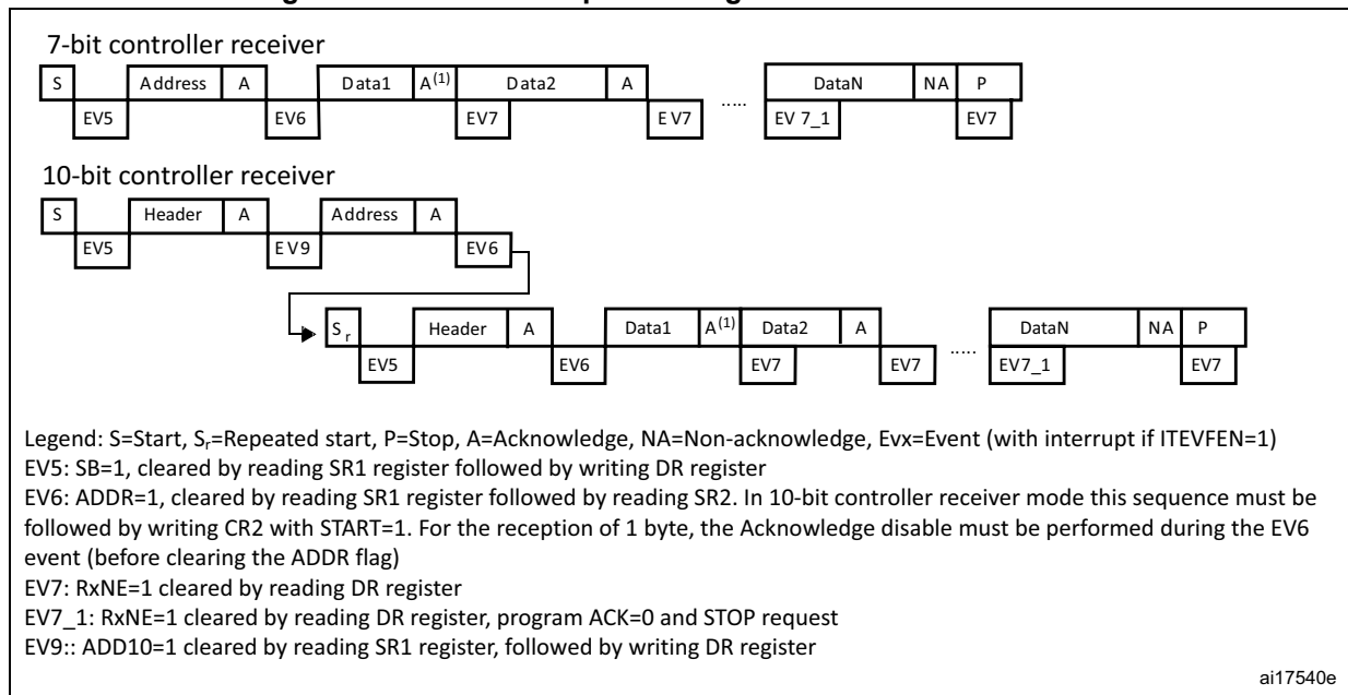
Figure 244. Transfer sequence diagram for controller receiver
