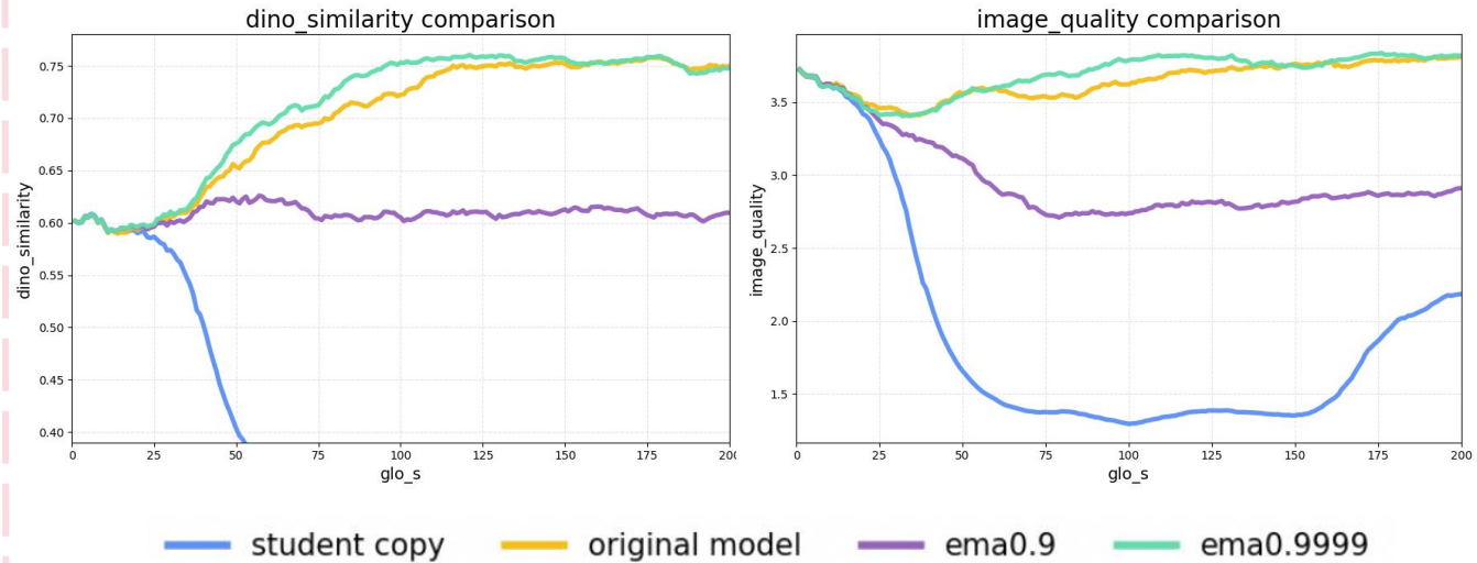
(b) Ablation on construction of the teacher model
