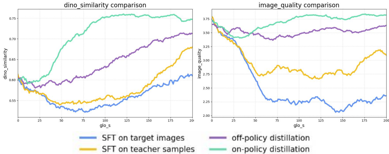
(a) Ablation on the training strategy
