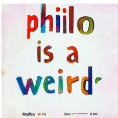
GRPO-GenEval
