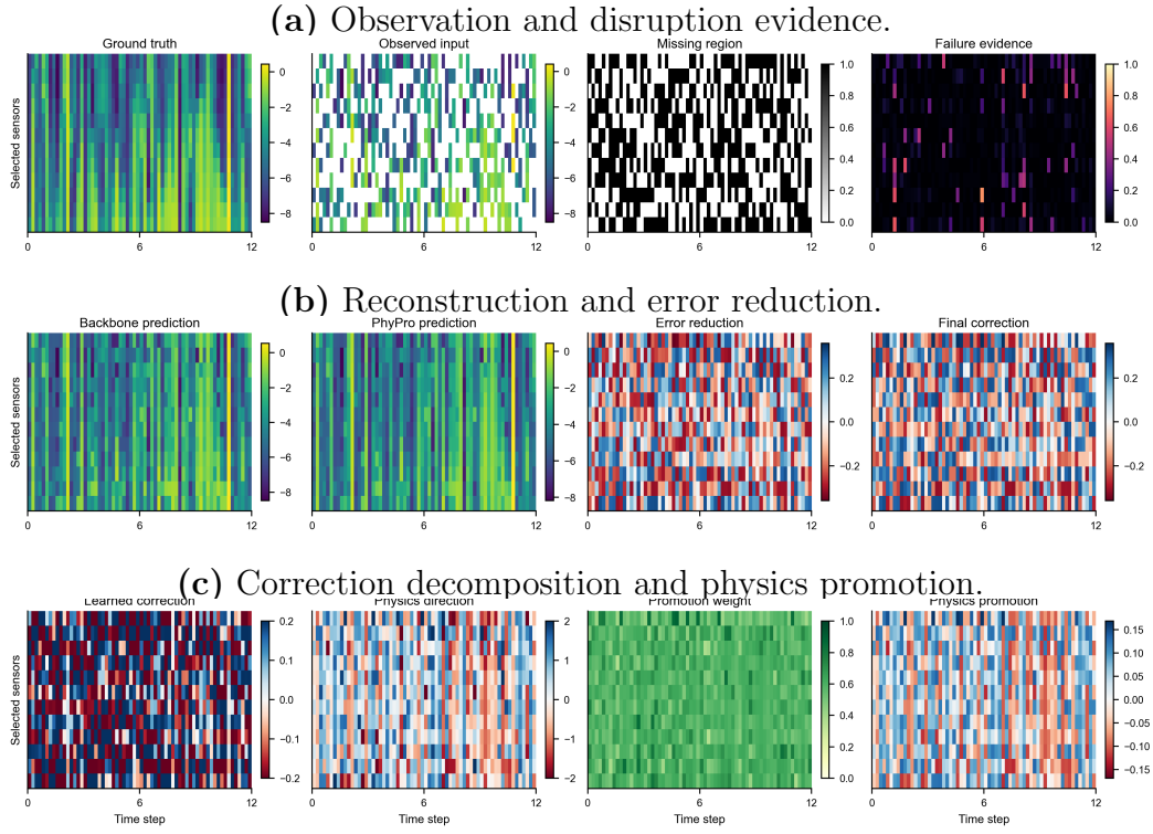
Figure 2: Representative PhyPro reconstruction case on PEMS-BAY under random missing with 50% missingness. PhyPro reduces masked MAE from 0.2457 to 0.2070 in this case.
