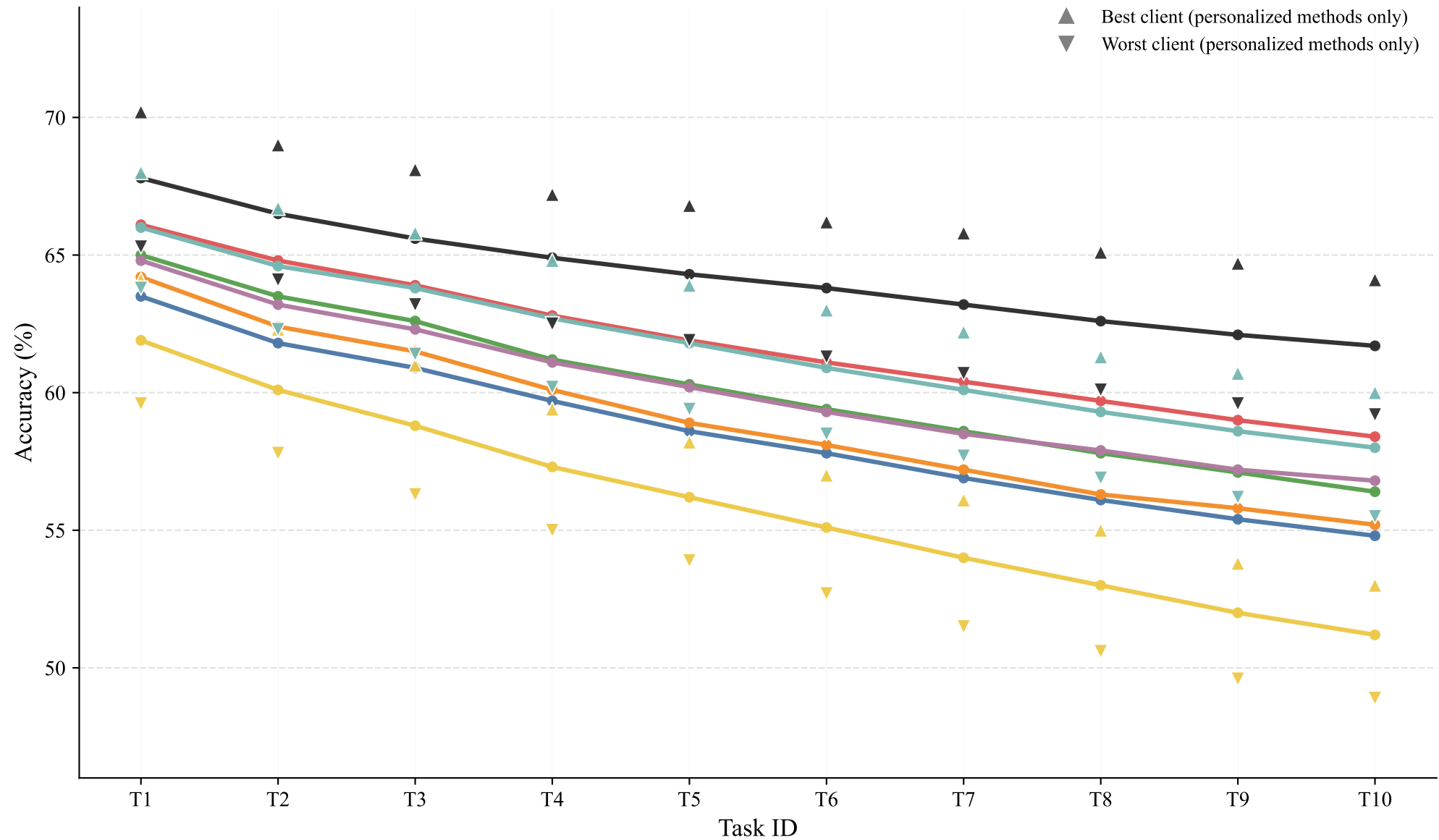
CIFAR-100 non-IID ( \alpha=0.3 ): Task-wise Accuracy Over 10 Tasks
