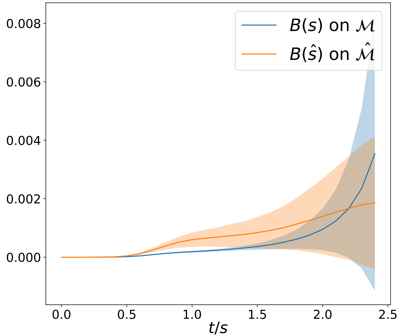
Barrier Value on \mathcal{M} & \hat{\mathcal{M}}
