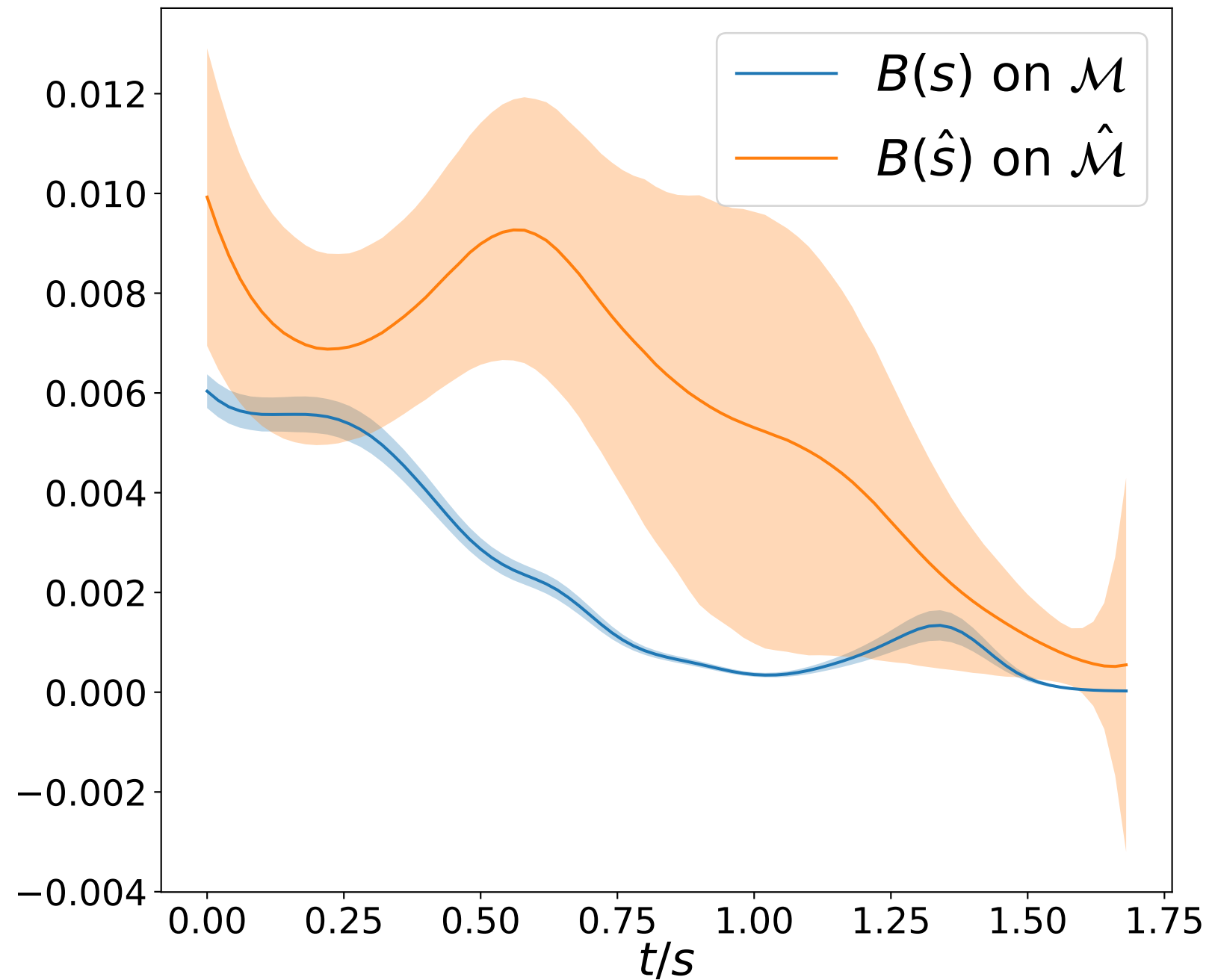
Barrier Value on \mathcal{M} & \hat{\mathcal{M}}
