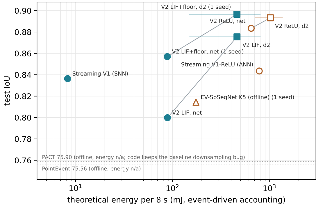
(a) test IoU at threshold 0.9 (benchmark protocol)
